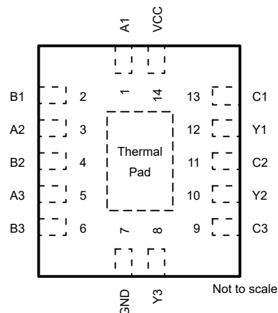
Figure 4-2. SN74LVC3G98 BQA Package, 14-Pin WQFN (Top View)
