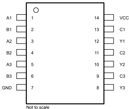
Figure 4-1. SN74LVC3G98 PW Package (Preview), 14-Pin TSSOP (Top View)
