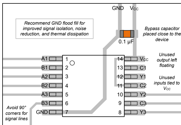
Figure 8-3. Example Layout for the SN74LVC3G98
