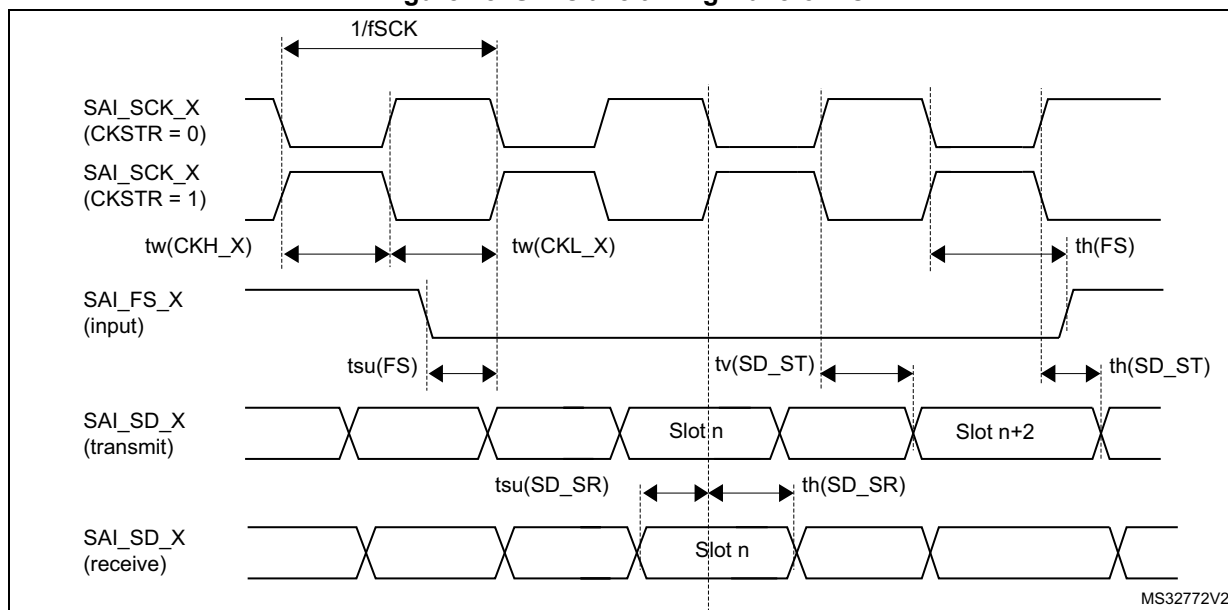
Figure 48. SAI slave timing waveforms
