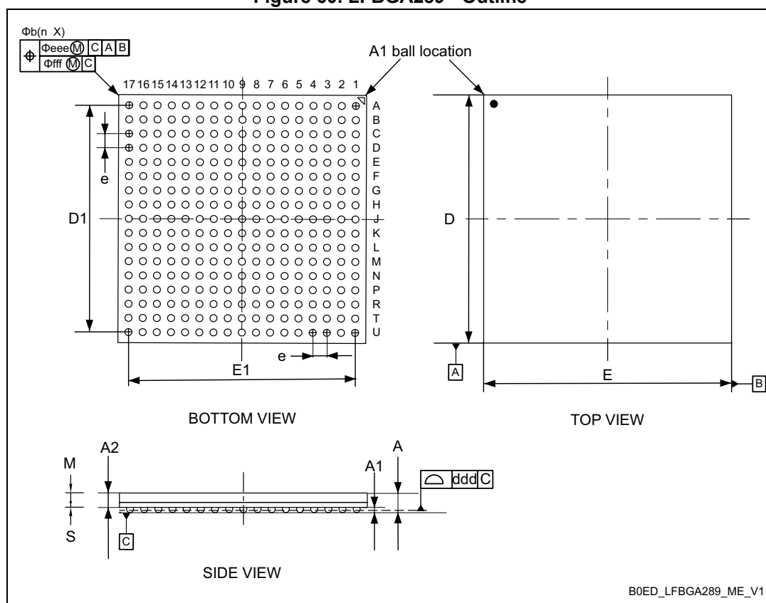
Figure 60. LFBGA289 - Outline
