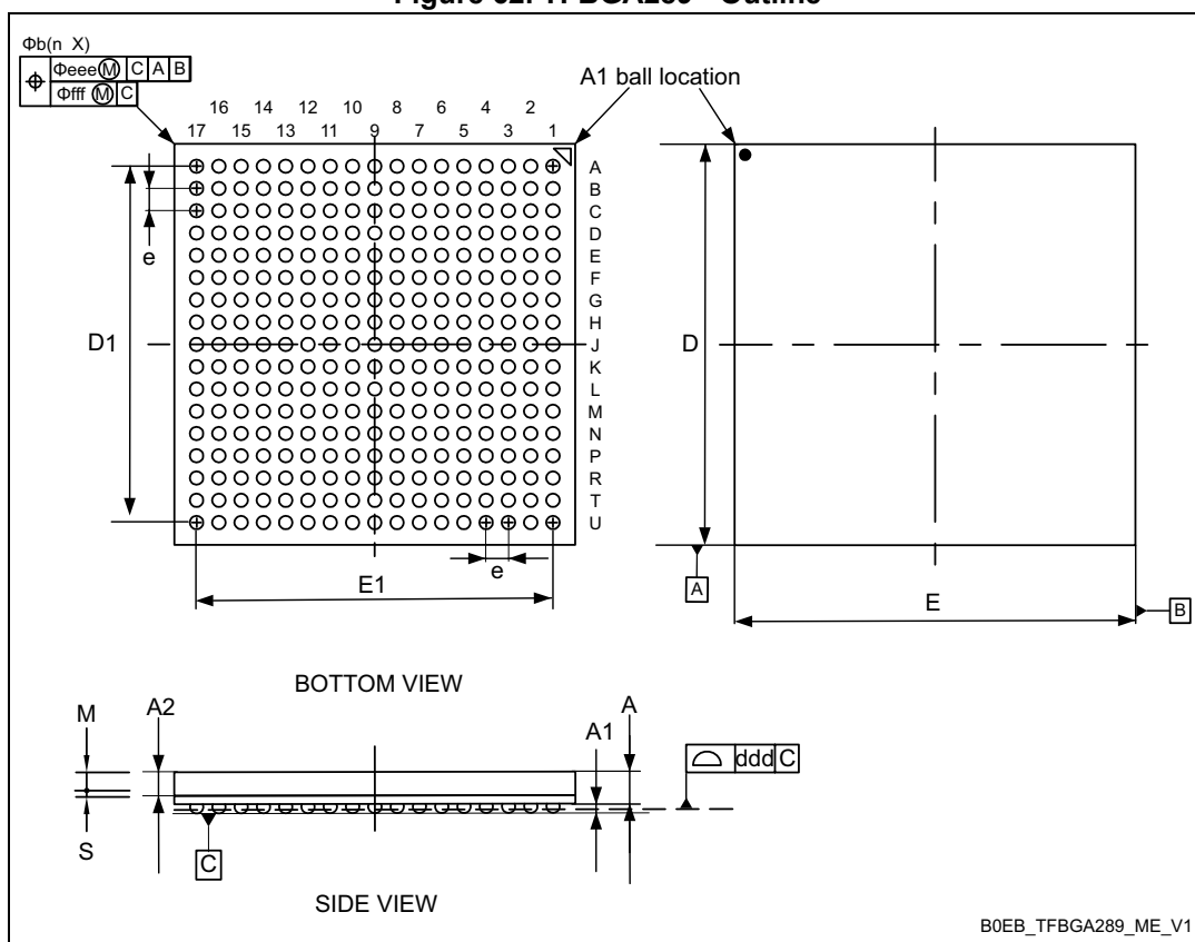
Figure 62. TFBGA289 - Outline
