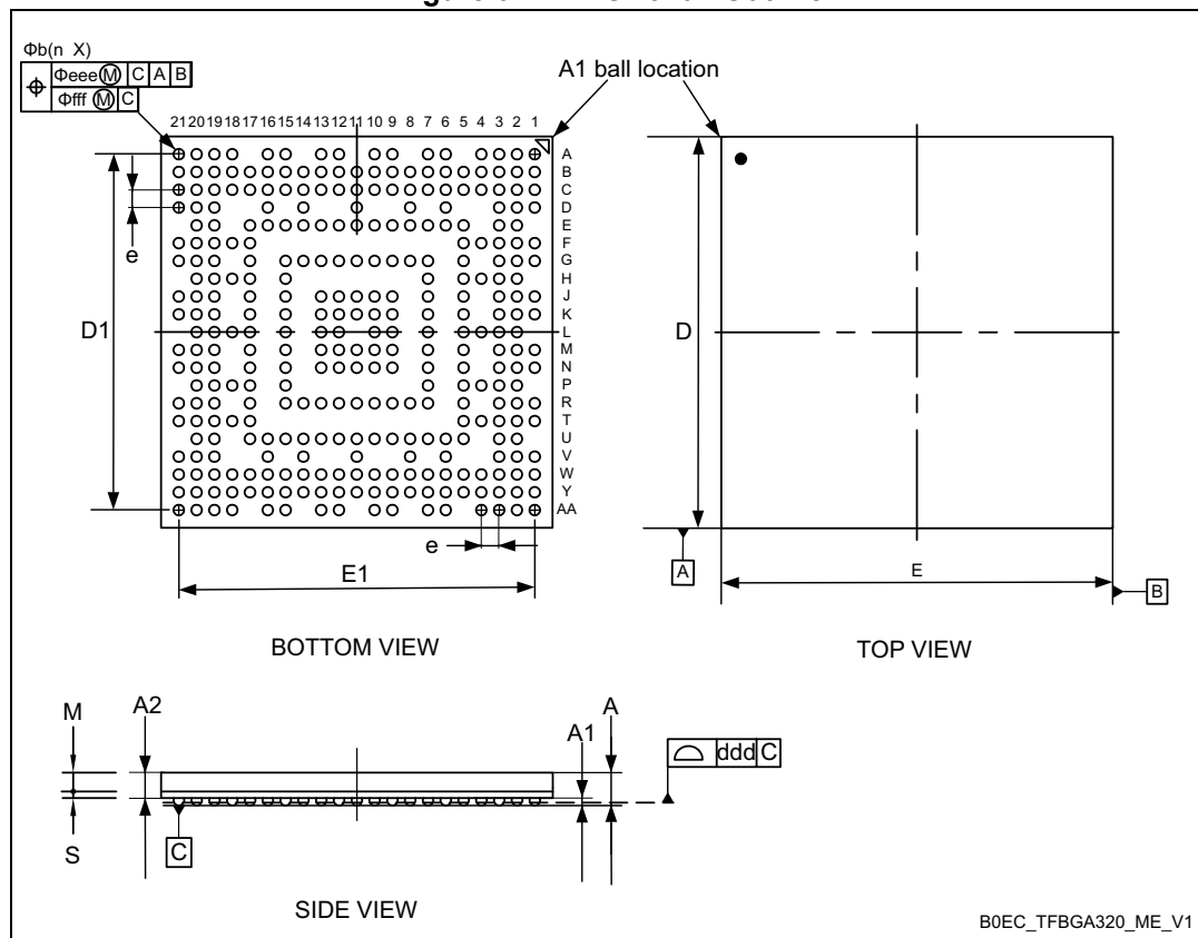
Figure 64. TFBGA320 - Outline
