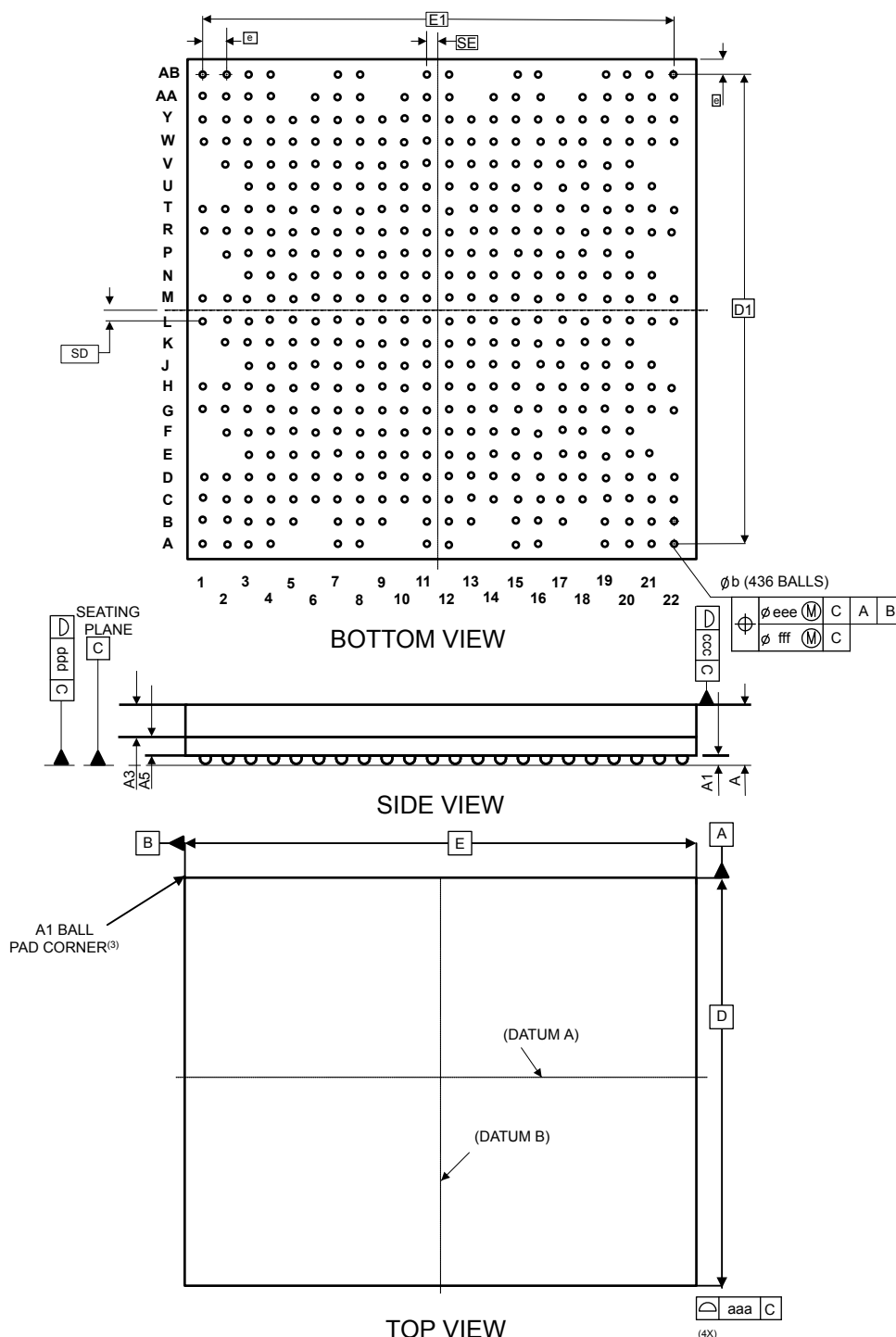
Figure 68. TFBGA436 - Outline
