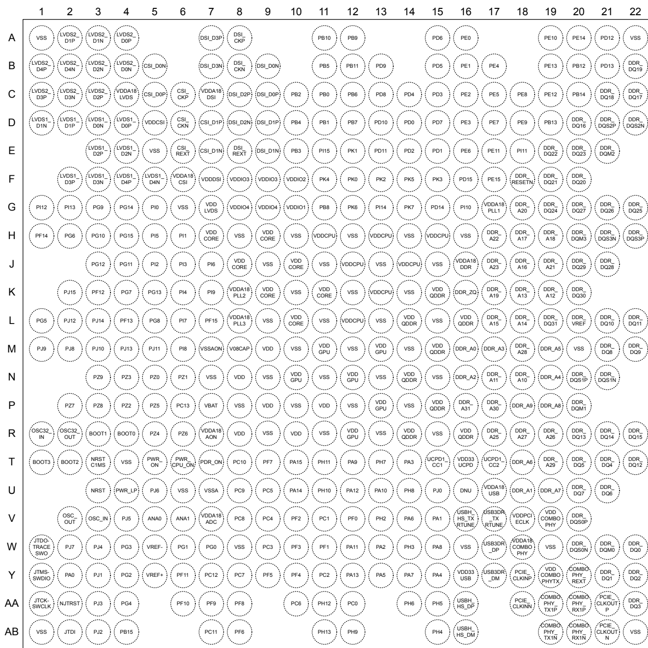
Figure 9. STM32MP25xA/D TFBGA436 ballout
