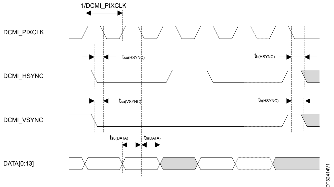
Figure 42. DCMI timing diagram
