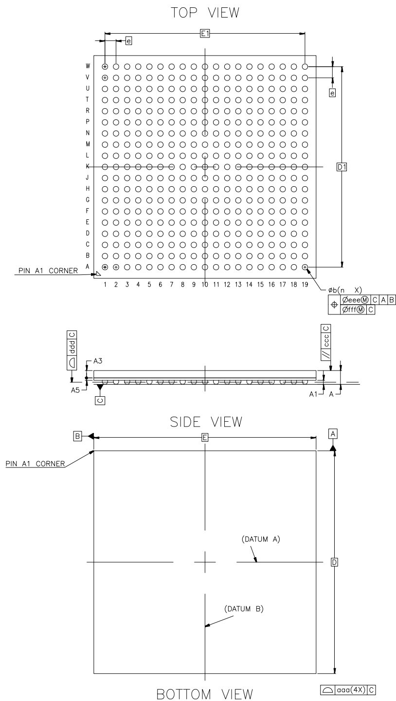
Figure 65. TFBGA361 - Outline
