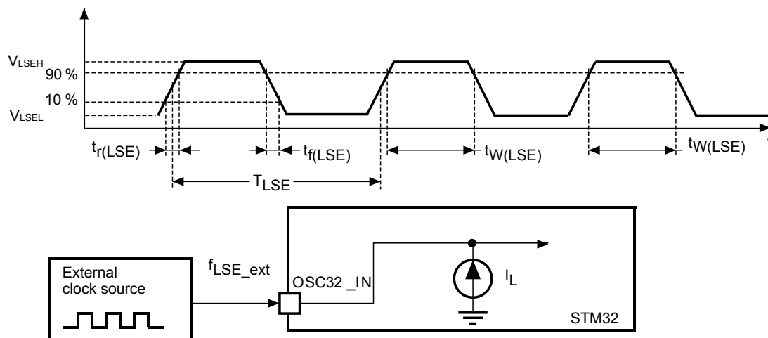
Figure 16. Low-speed external clock source AC timing diagram (digital bypass)
