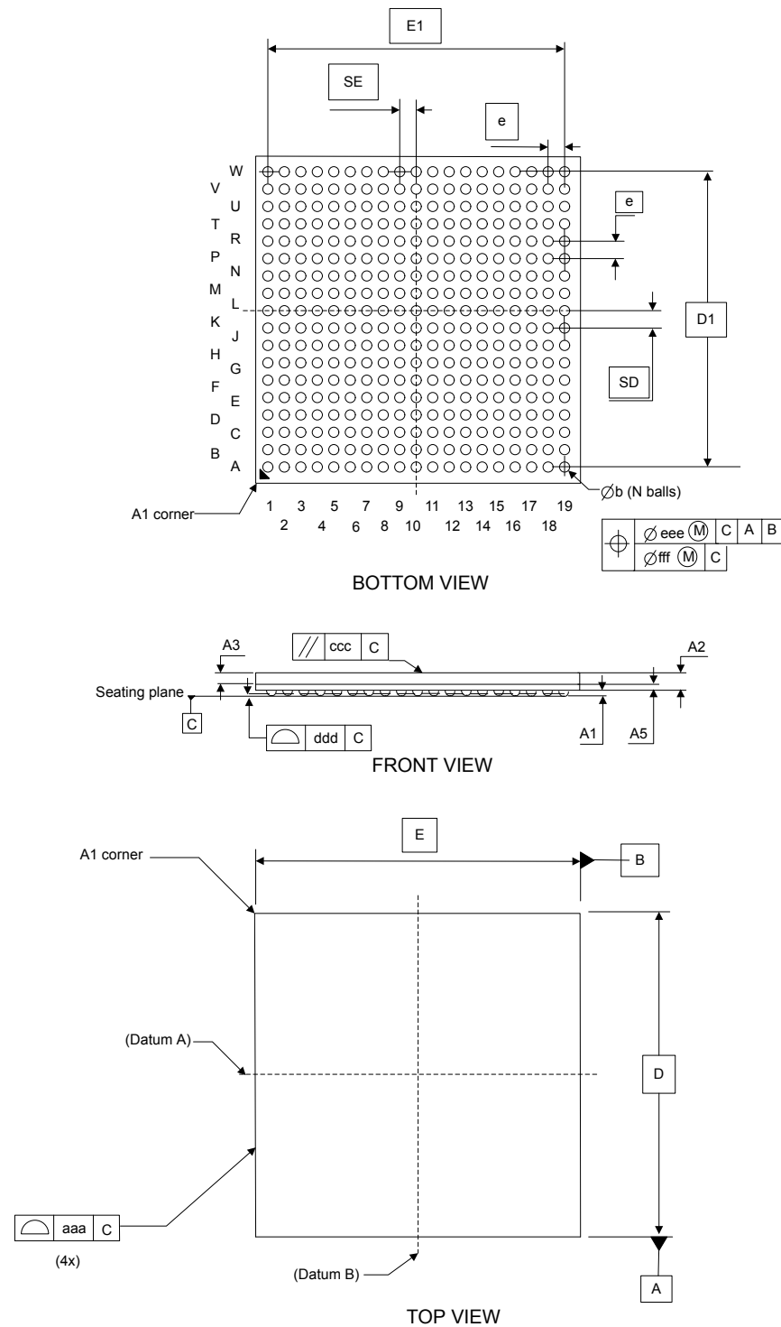
Figure 66. VFBGA361 - Outline
