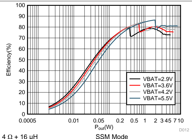
Figure 18. Efficiency vs Output Power High Efficiency
