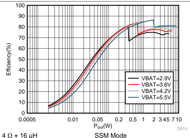
Figure 16. Efficiency vs Output Power Low Inrush
