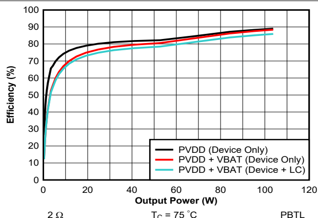
Figure 7-33. Efficiency vs Output Power - PBTL - 2 \Omega
