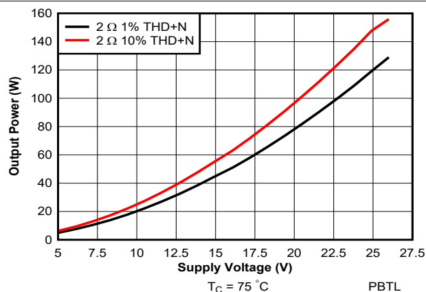
Figure 7-32. Output Power vs Supply Voltage - PBTL
