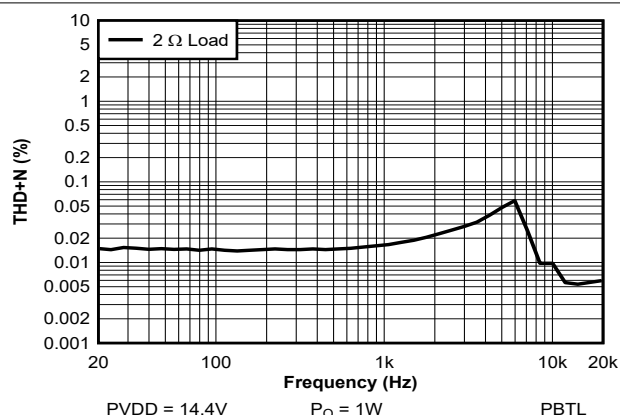
Figure 7-30. THD+N vs Frequency - PBTL - 14.4 V
