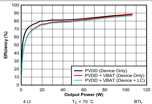
Figure 7-6. Efficiency vs Output Power - 14.4 V - 4 \Omega
