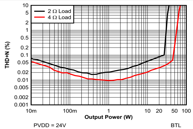
Figure 7-2. THD+N vs Power - 24V
