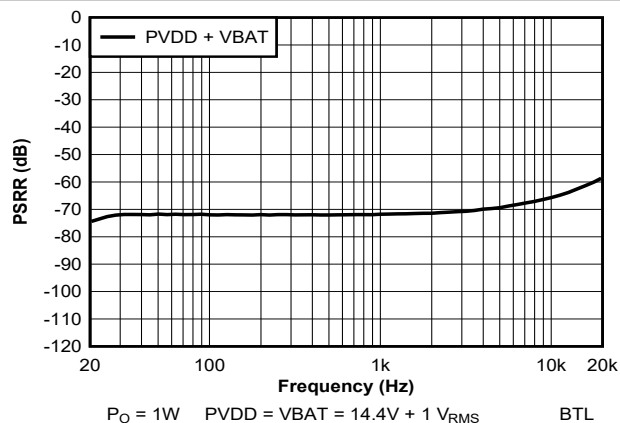
Figure 7-18. PSRR vs Frequency - PVDD + VBAT
