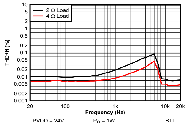
Figure 7-4. THD+N vs Frequency - 24 V
