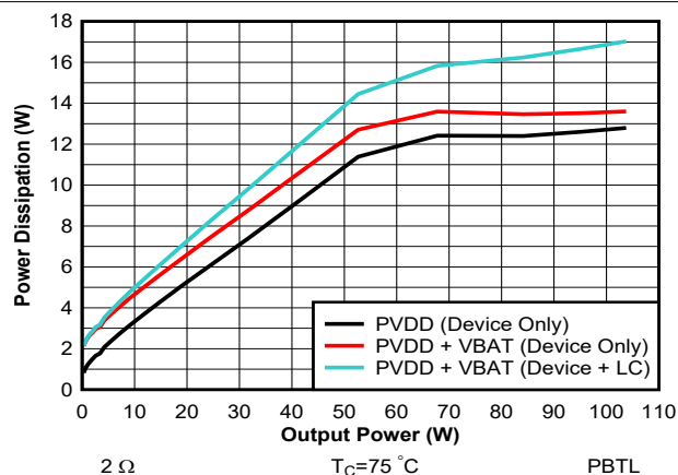
Figure 7-35. Power Dissipation vs Output Power - PBTL - 2 \Omega
