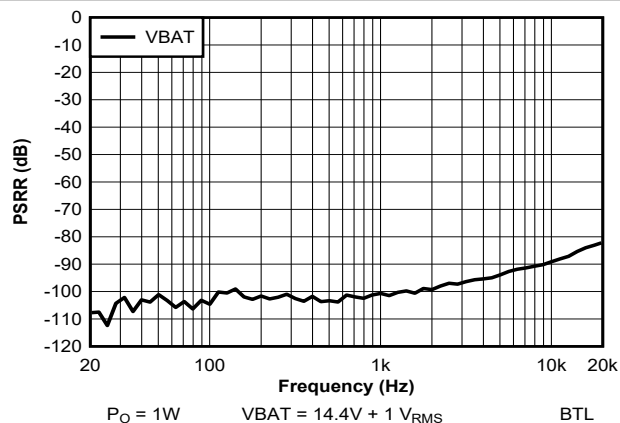
Figure 7-17. PSRR vs Frequency - VBAT Only
