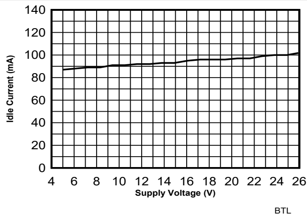
Figure 7-13. VBAT Idle Current vs Supply Voltage
