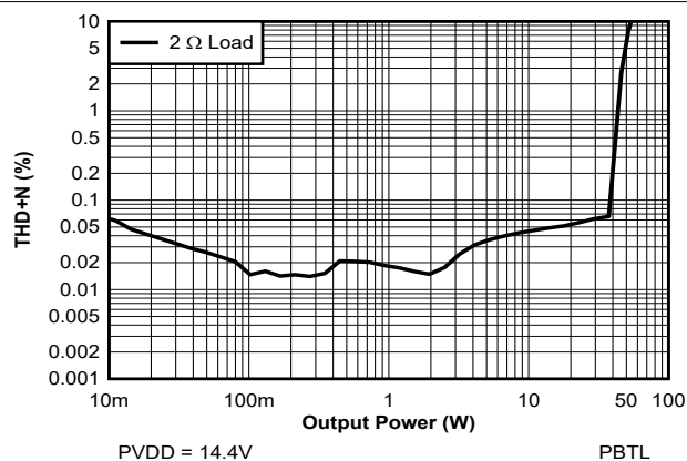
Figure 7-28. THD+N vs Power - PBTL - 14.4V
