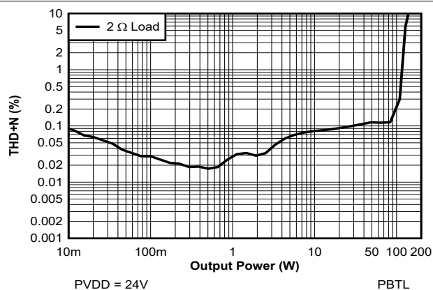
Figure 7-29. THD+N vs Power - PBTL - 24 V
