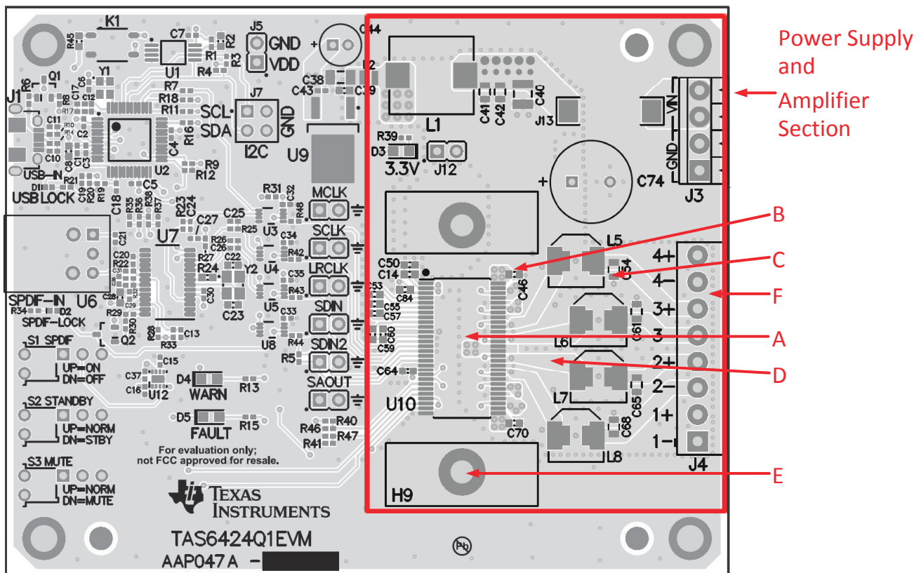
Figure 10-4. EVM Layout
