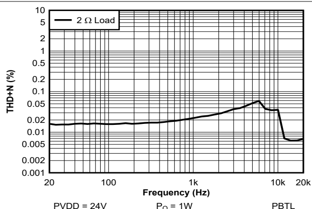
Figure 7-31. THD+N vs Frequency - PBTL - 24 V
