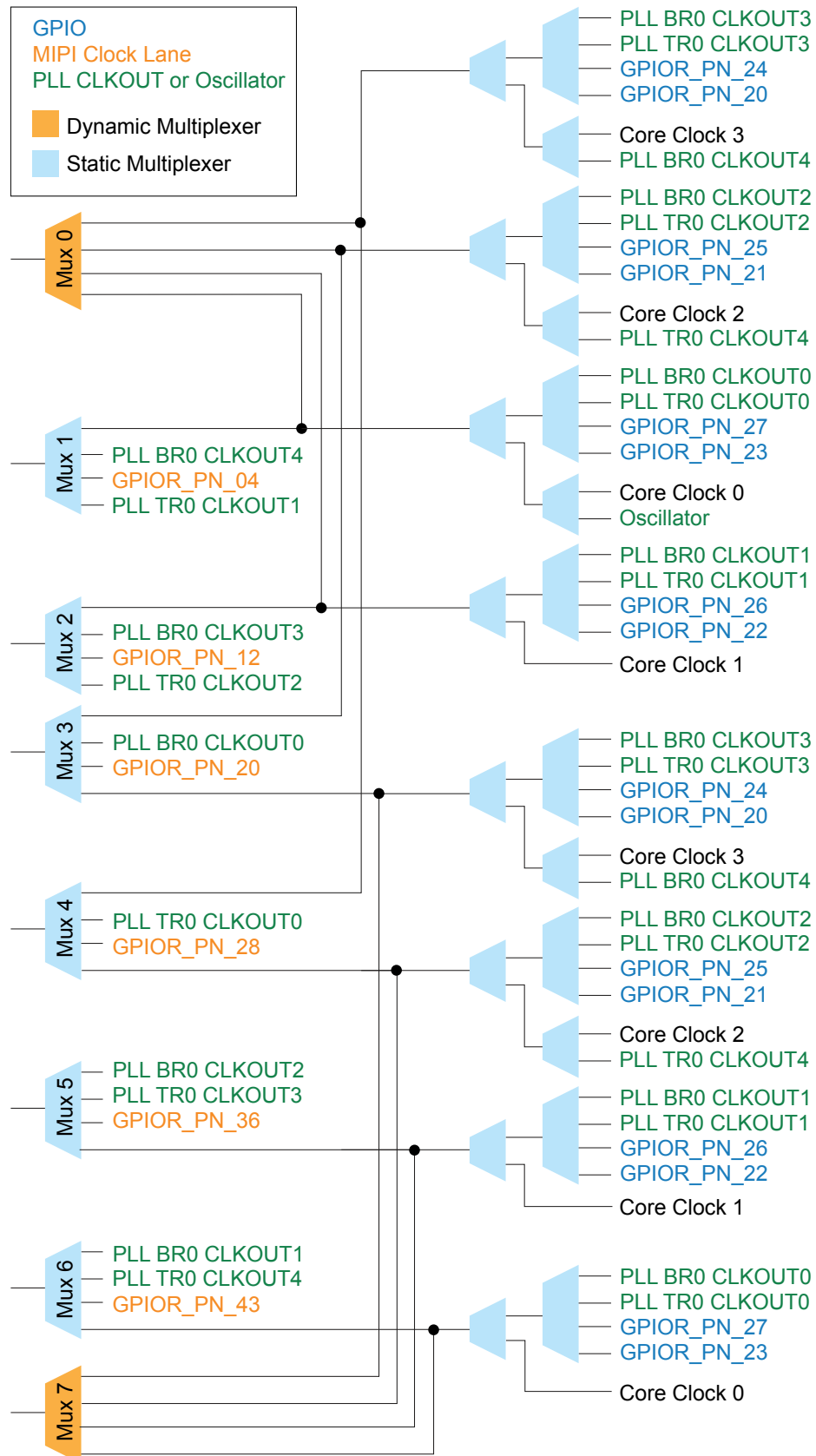
Figure 11: Clock Sources that Drive the Multiplexers: Right
