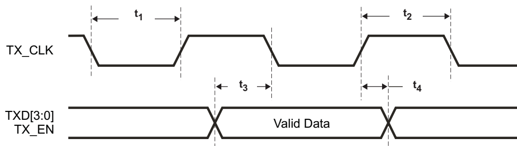
Figure 9-11. 10 Mb/s MII Transmit Timing
