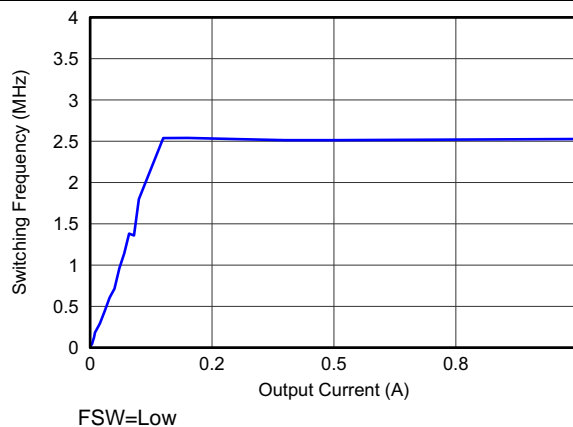
Figure 23. Switching Frequency
