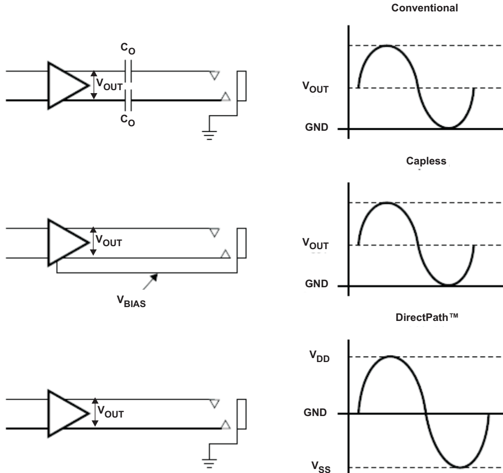
Figure 31. Amplifier Applications
