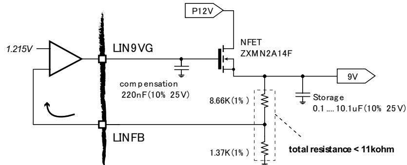
Figure 63. Example Circuit of 9-V LDO
