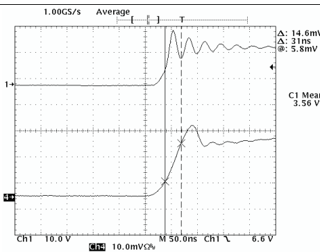
Figure 6. Input Current With Slope Control
