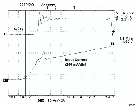
Figure 2. Low-Power-Mode Current, I_O = 0 \text{ mA} - 1 \text{ mA}
