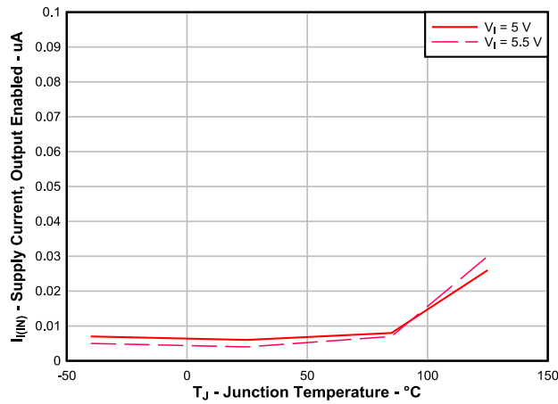
Figure 6-31. TPS2051BDBV Supply Current, Output Disabled vs Junction Temperature
