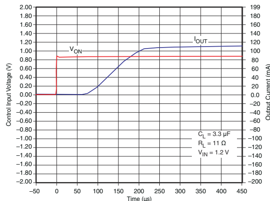
Figure 7-24. t_{ON} Response
