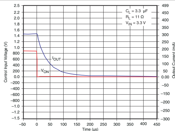
Figure 7-28. t_{OFF} Response
