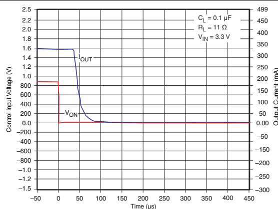
Figure 7-26. t_{OFF} Response
