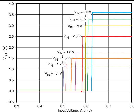
Figure 10. ON-Input Threshold
