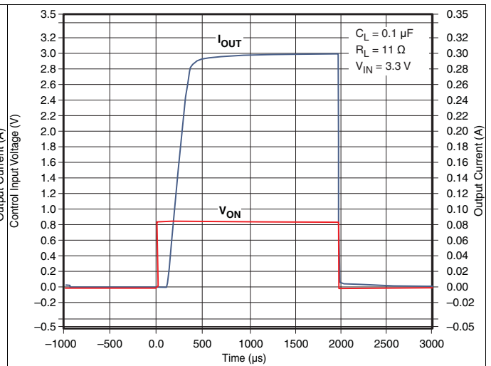
Figure 14. t_{ON} Response
