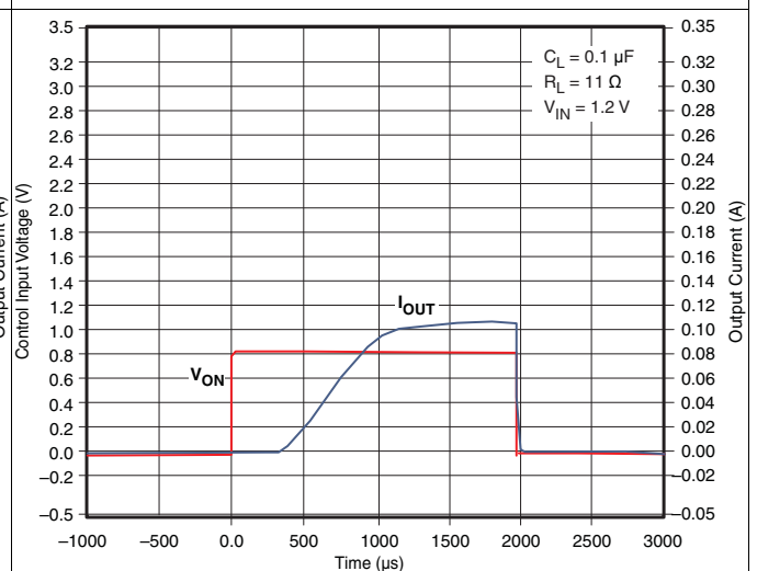
Figure 18. t_{ON} Response
