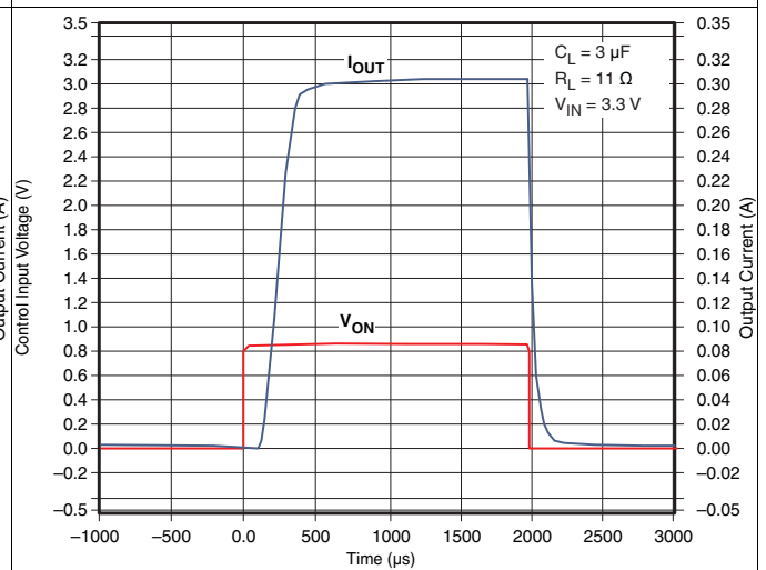
Figure 16. t_{ON} Response
