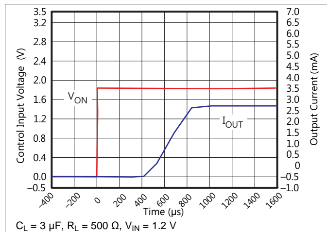
Figure 19. t_{ON} Response
