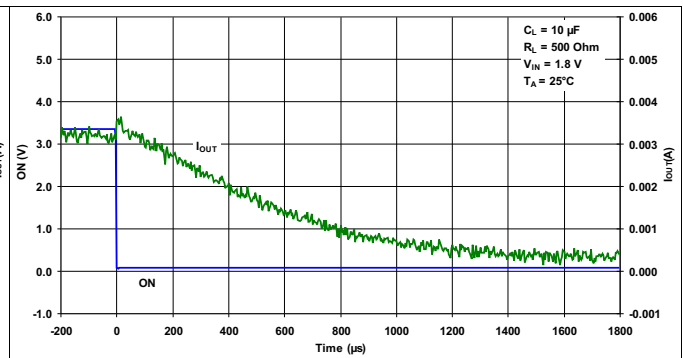
Figure 20. t_{OFF} Response
