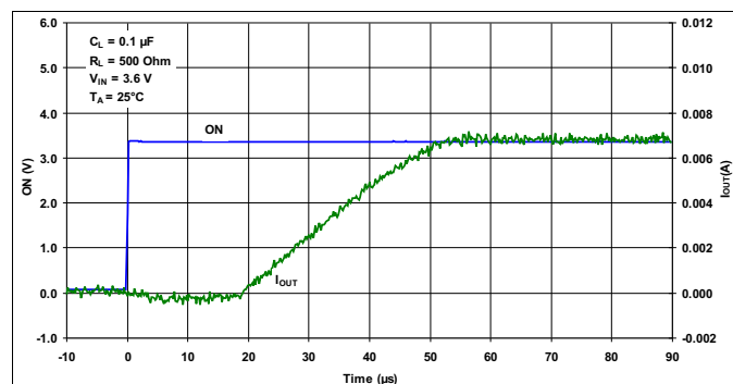
Figure 13. t_{ON} Response
