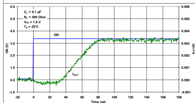
Figure 15. t_{ON} Response
