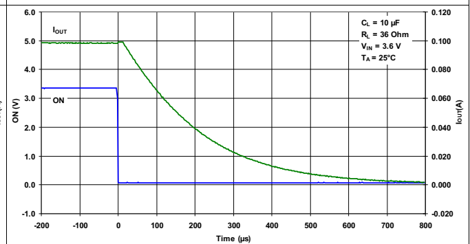
Figure 22. t_{OFF} Response
