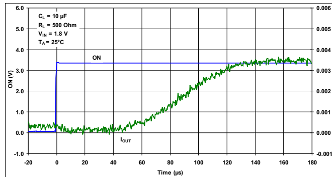
Figure 19. t_{ON} Response
