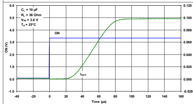
Figure 21. t_{ON} Response
