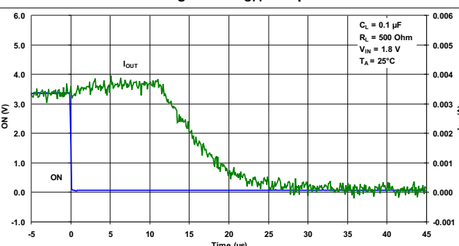
Figure 16. t_{OFF} Response
