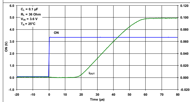
Figure 19. t_{ON} Response
