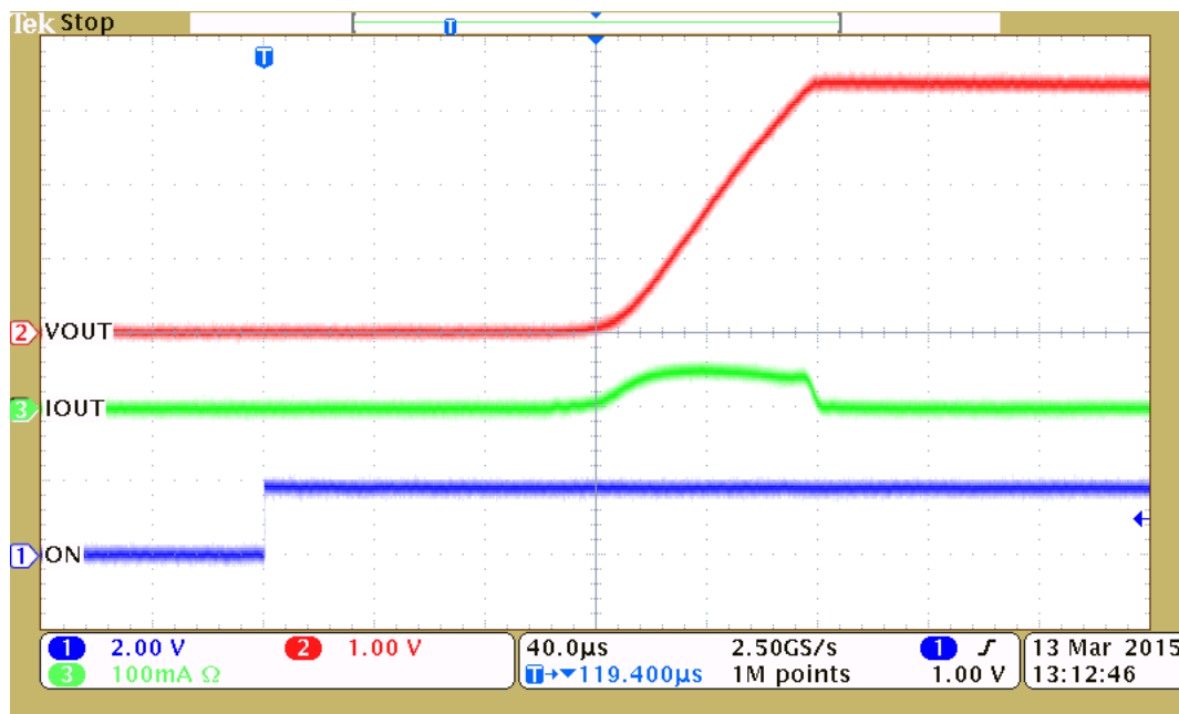
Figure 35. Inrush Current With 1- \mu F Output Capacitor
