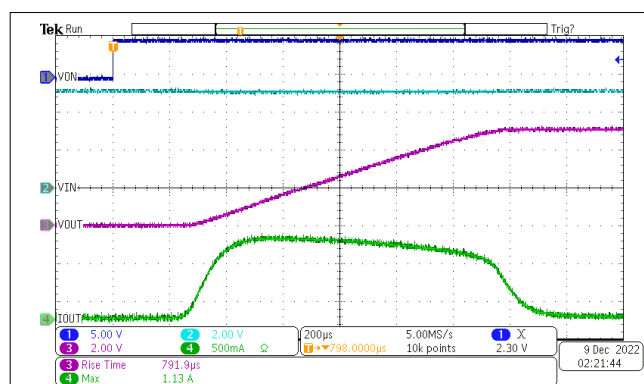
Figure 9-2. Inrush Current for C_L = 220 \text{ } \mu\text{F} with C_T = 1000 \text{ pF}
