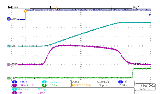
Figure 9-3. PG Pin Behavior with Inrush Current for C_L = 220 \text{ } \mu\text{F} with C_T = 1000 \text{ pF}
