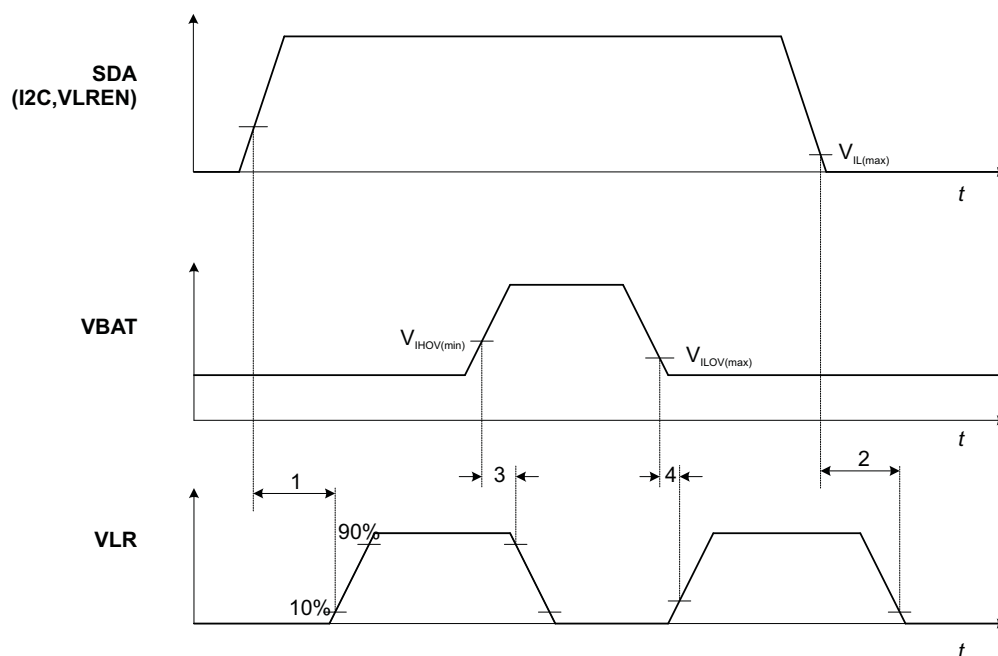
Figure 5. Linear Regulator Timing
