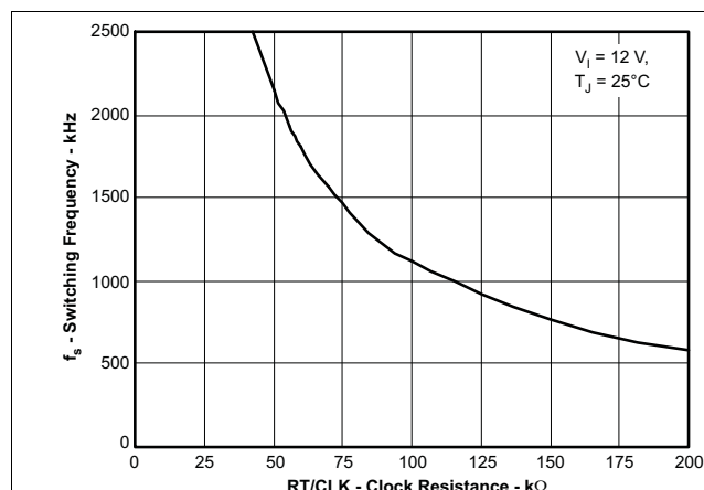
Figure 31. High-Range RT
