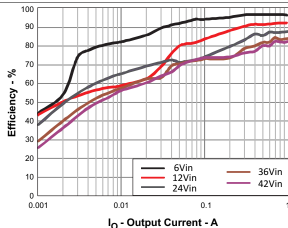
Figure 47. Light-Load Efficiency
