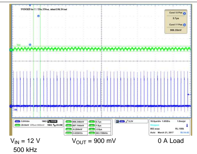
Figure 8. Output Voltage Ripple at Steady State
