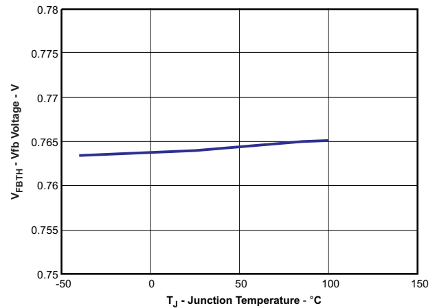
Figure 4. VFB Voltage vs Junction Temperature
