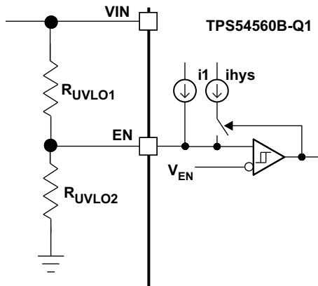
Figure 22. Adjustable Undervoltage Lockout (UVLO)
