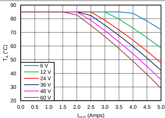
Figure 52. 3.3 V Outputs
