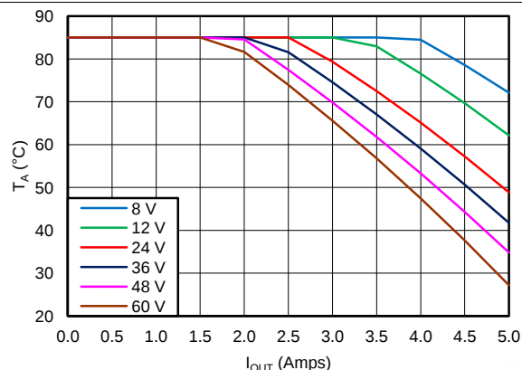
Figure 53. 5 V Outputs
