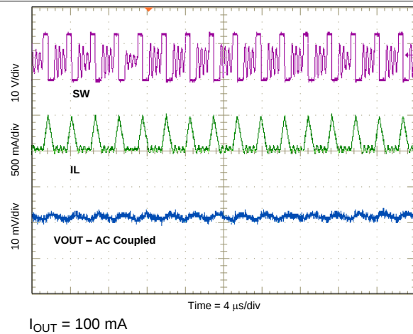
Figure 39. Output Ripple DCM
