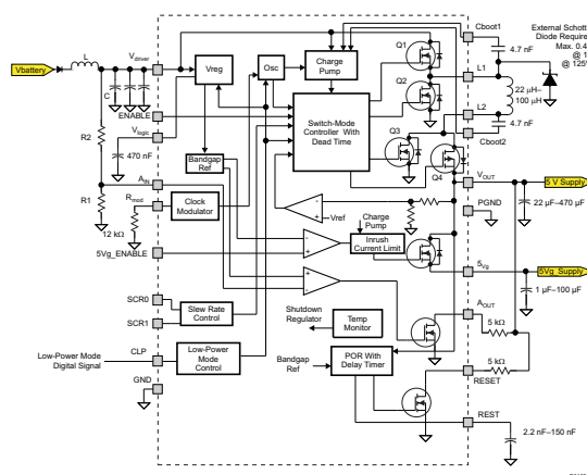
Simplified Schematic
