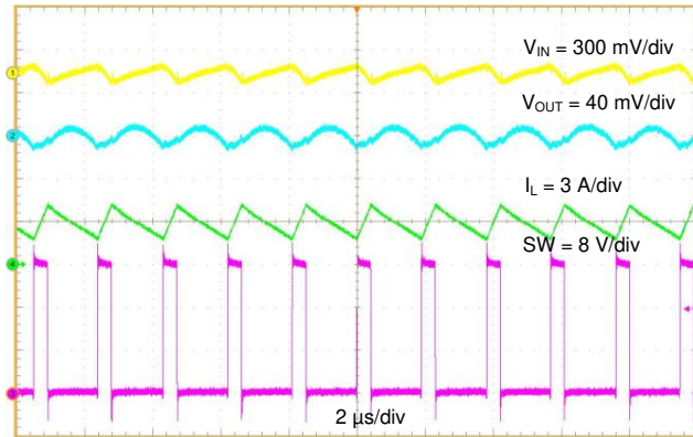
Figure 24. Steady State Waveforms, I_{OUT} = 3 A
