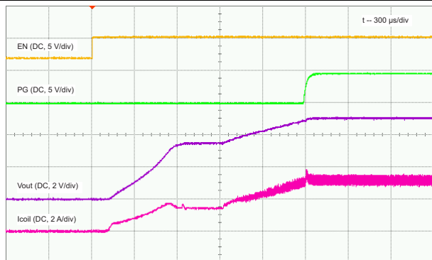
Figure 23. Startup ( V_{OUT} = 5\text{ V} , R_{OUT} = 2.5\text{ }\Omega )
