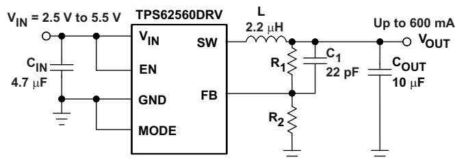
Figure 6. TPS62560DRV Adjustable
