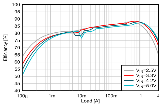
Figure 8-11. Efficiency versus Output Current
