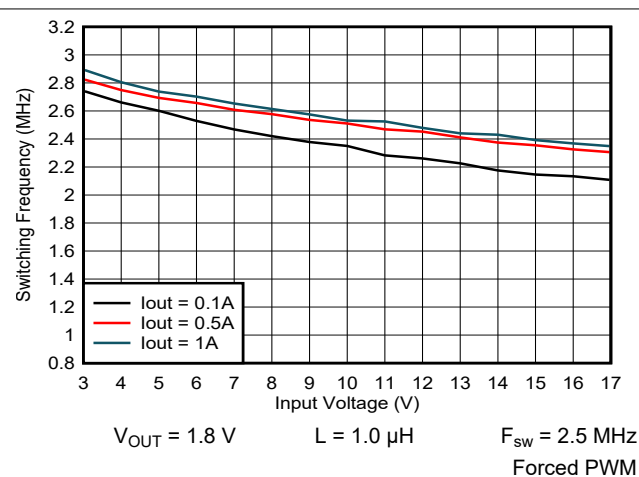
Figure 9-6. Switching Frequency vs Input Voltage
