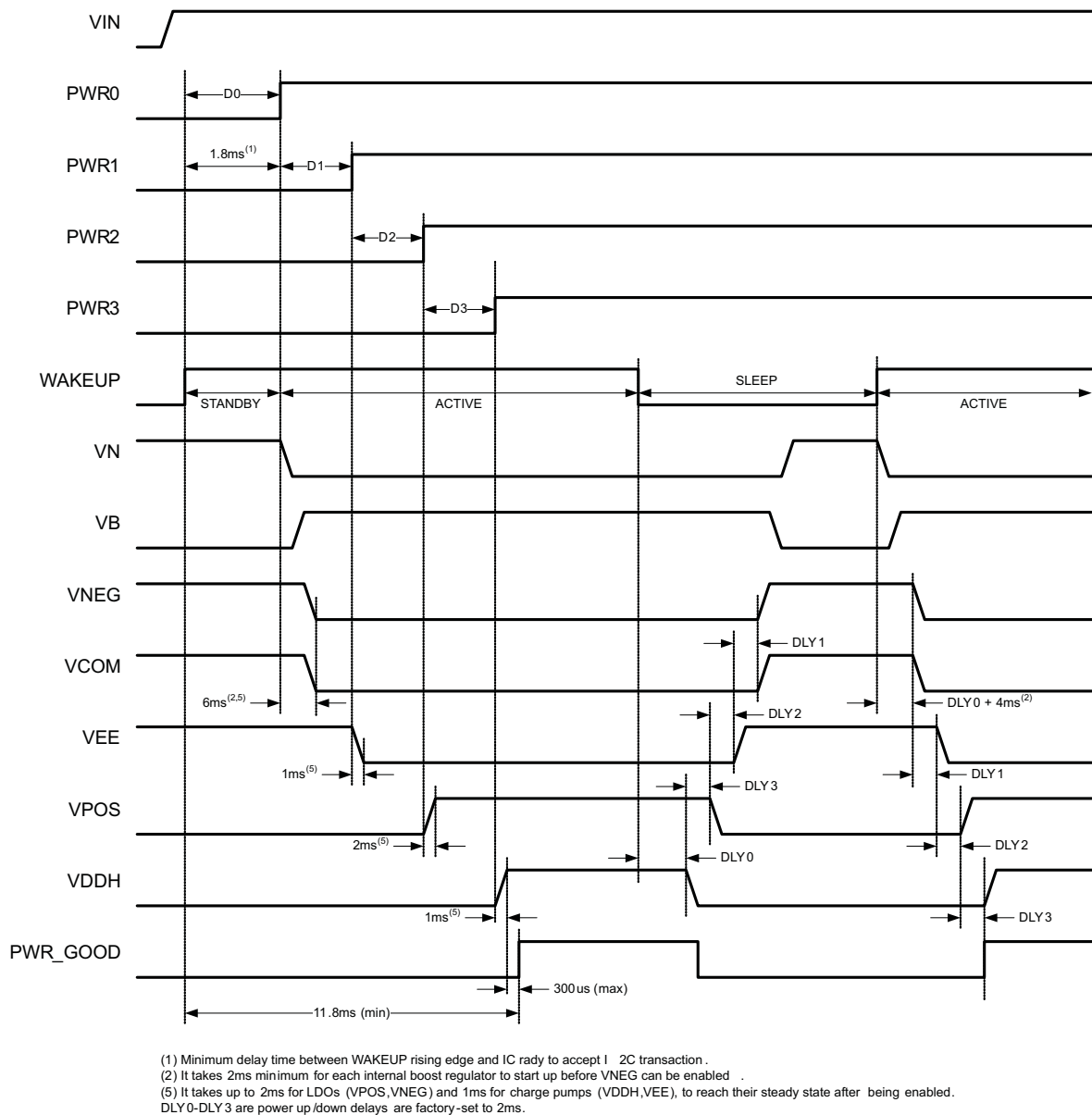
Figure 4. Power-Up and Power-Down Timing Diagram
