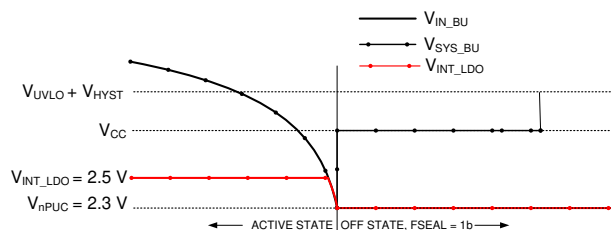
Figure 8-17. Switching Behavior of the Battery-Backup-Supply Power-Path; Power-Path Hysteresis
