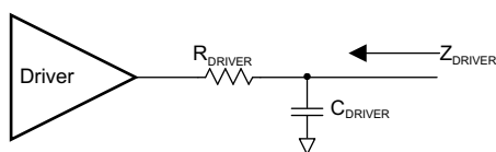
Figure 8-7. ZDRIVER Circuit
