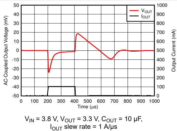
Figure 8-9. I_{OUT} Transient From 1 mA to 100 mA
