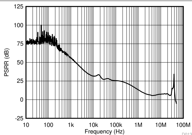
I_{OUT} = 100\text{ mA} Figure 6-13. PSRR vs Frequency
