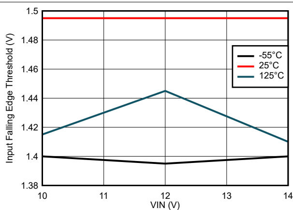
Figure 7-17. Input Falling Edge Threshold vs VIN Voltage
