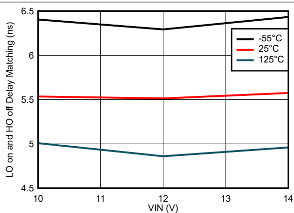
Figure 7-18. LO on and HO off Delay Matching vs VIN Voltage
