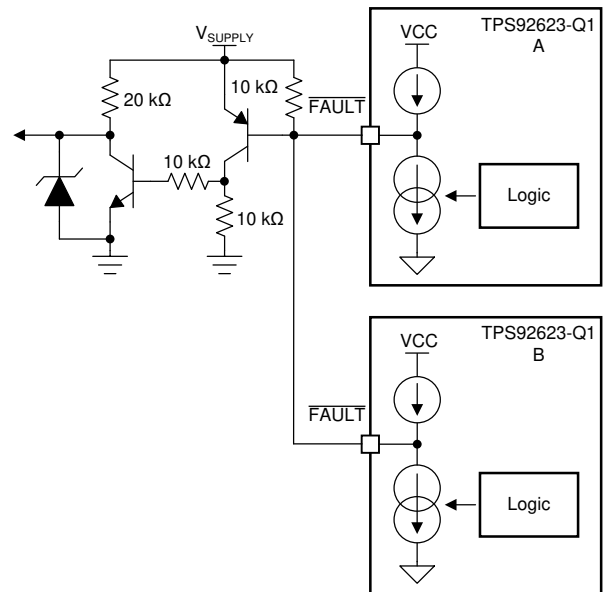
Figure 7-7. FAULT Bus for One-Fails-Others-On Application
