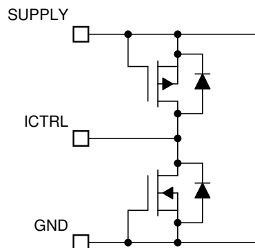
Figure 7-18. ICTRL pin
