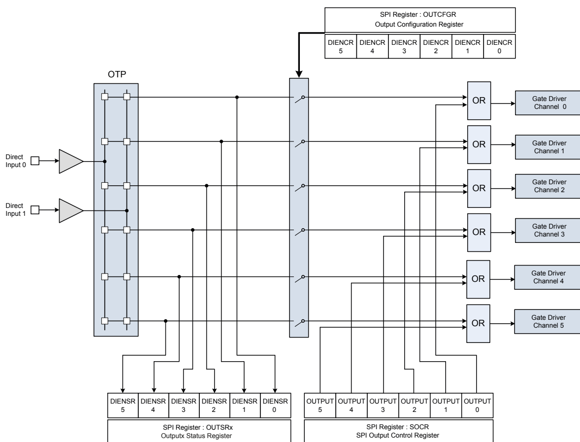
Figure 20. Direct input block diagram - valid for 2, 4 and 6 channels device
