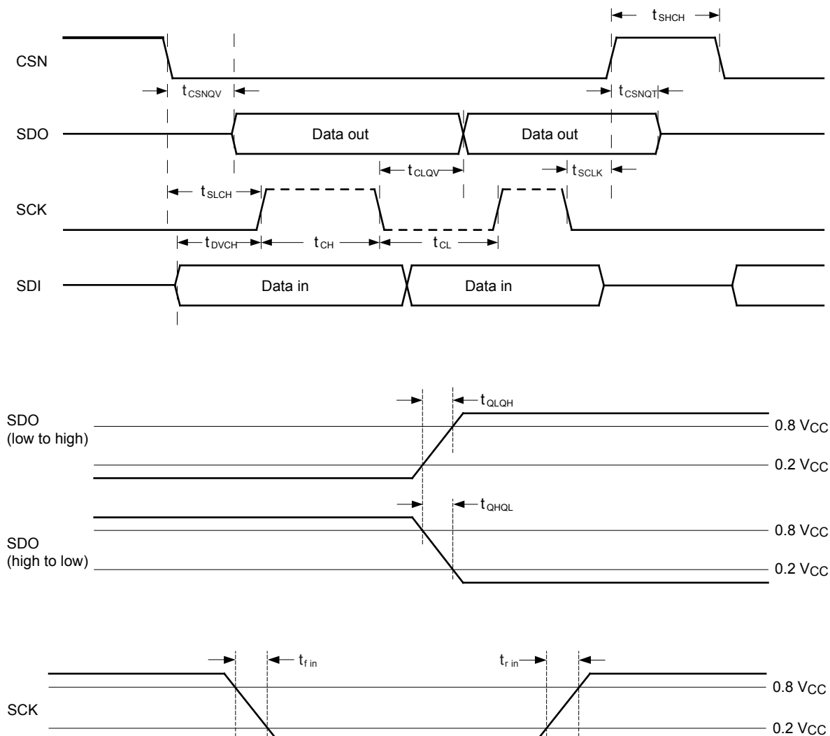
Figure 35. SPI dynamic characteristics
