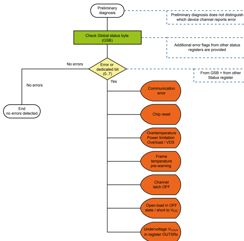
Figure 28. Status registers
