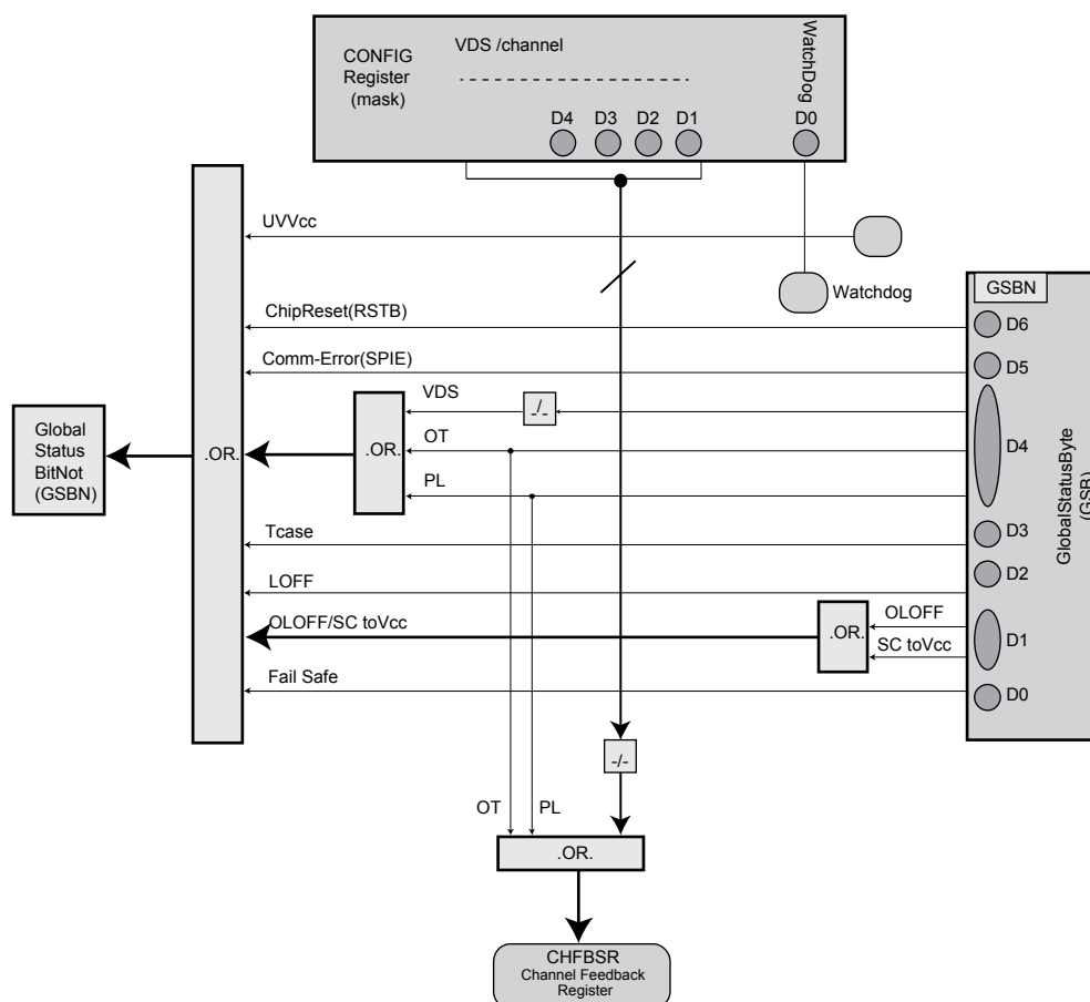
Figure 27. Diagnostic registers
