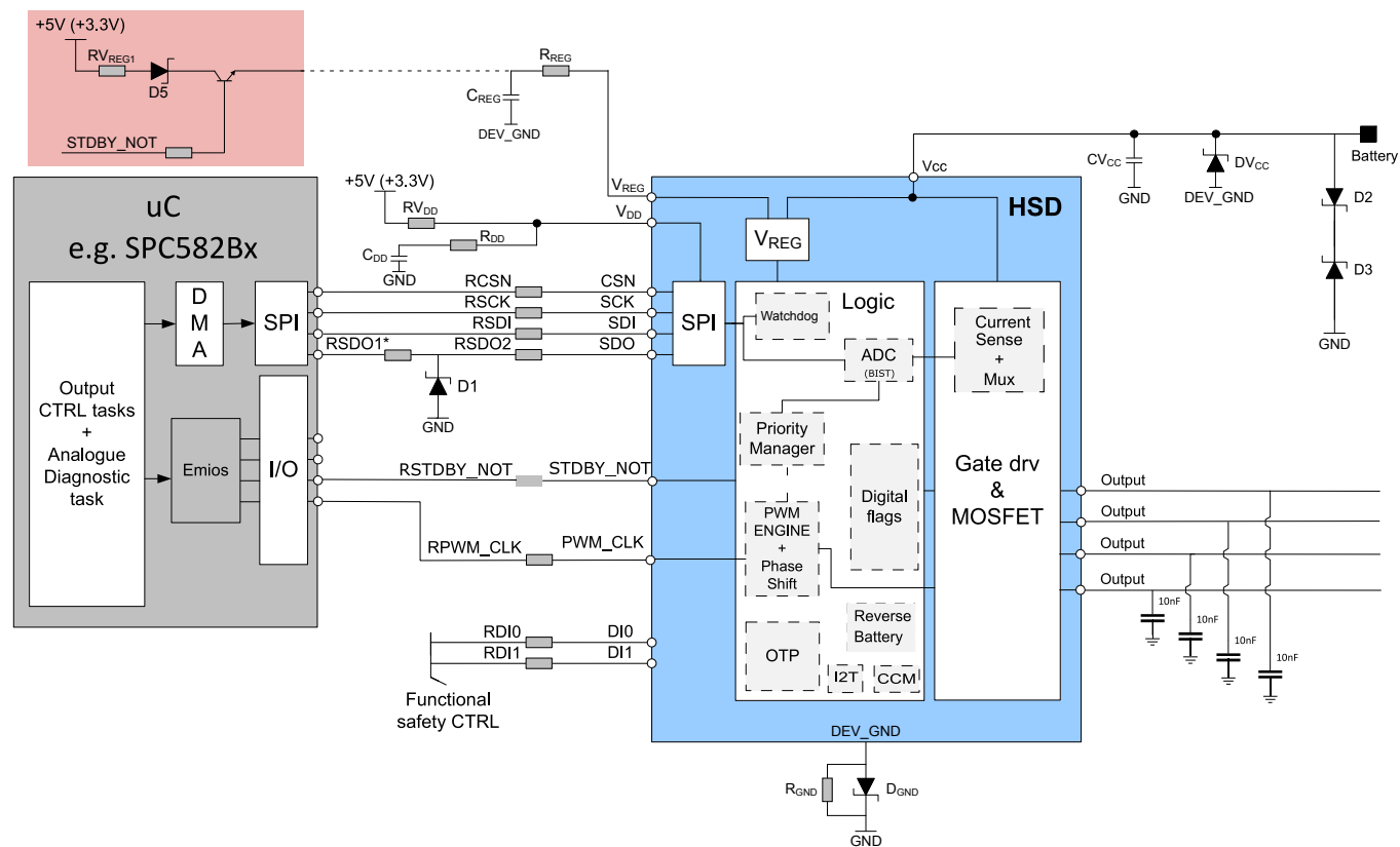
Figure 37. Application schematic
