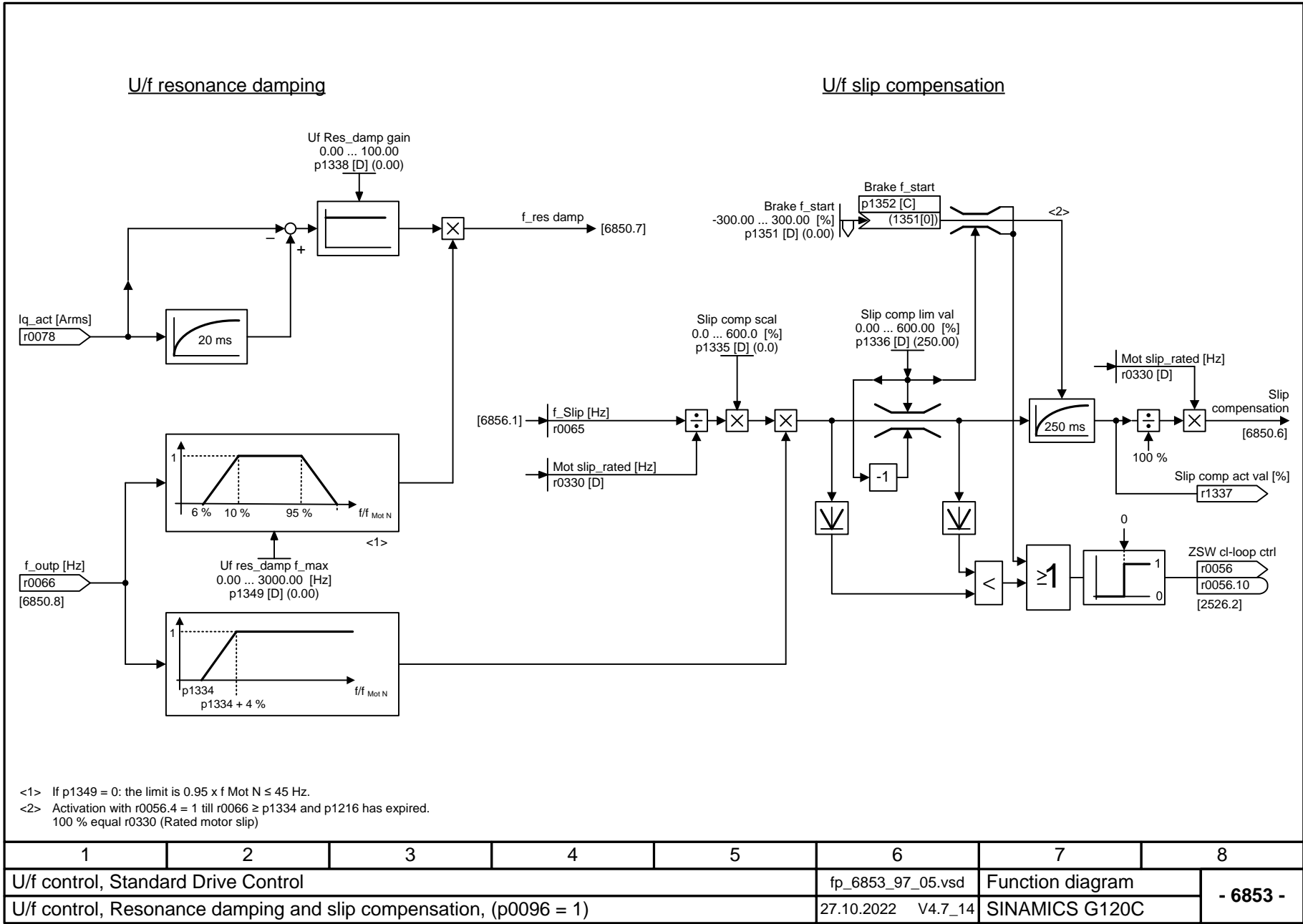
Fig. 3-102 6853 – U/f control, resonance damping and slip compensation (p0096 = 1)
