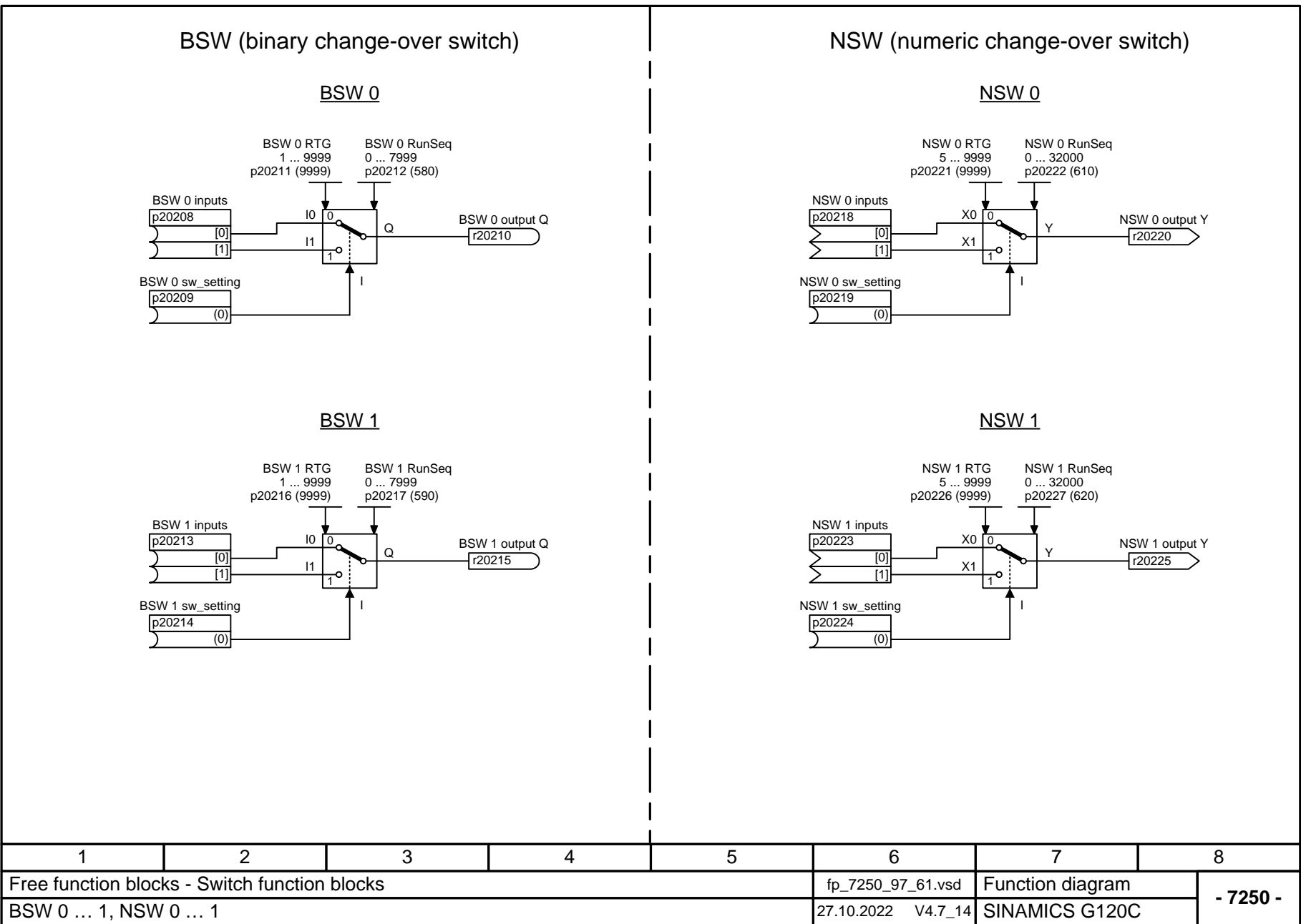
Fig. 3-141 7250 – BSW 0 ... 1, NSW 0 ... 1
