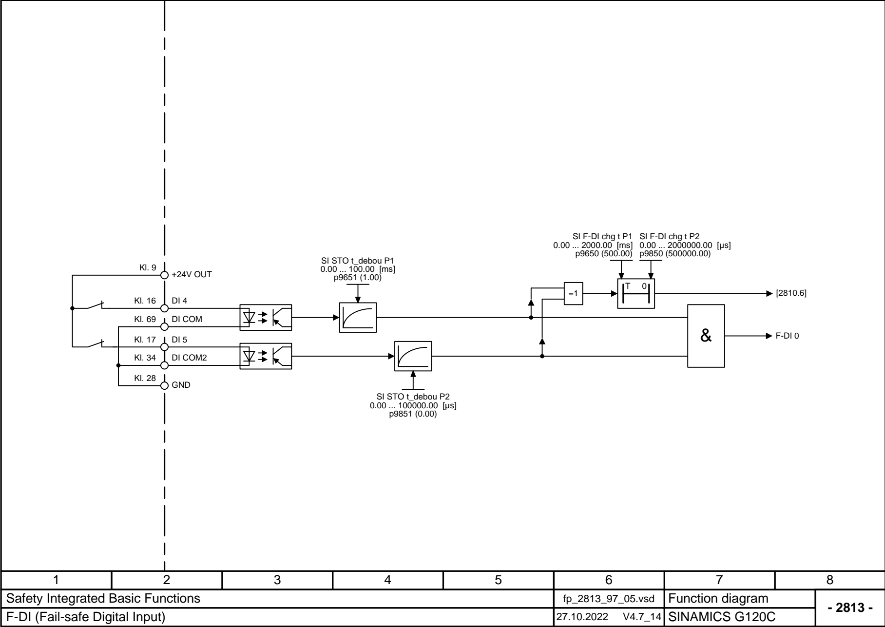
Fig. 3-62 2813 – F-DI (Fail-safe Digital Input)
