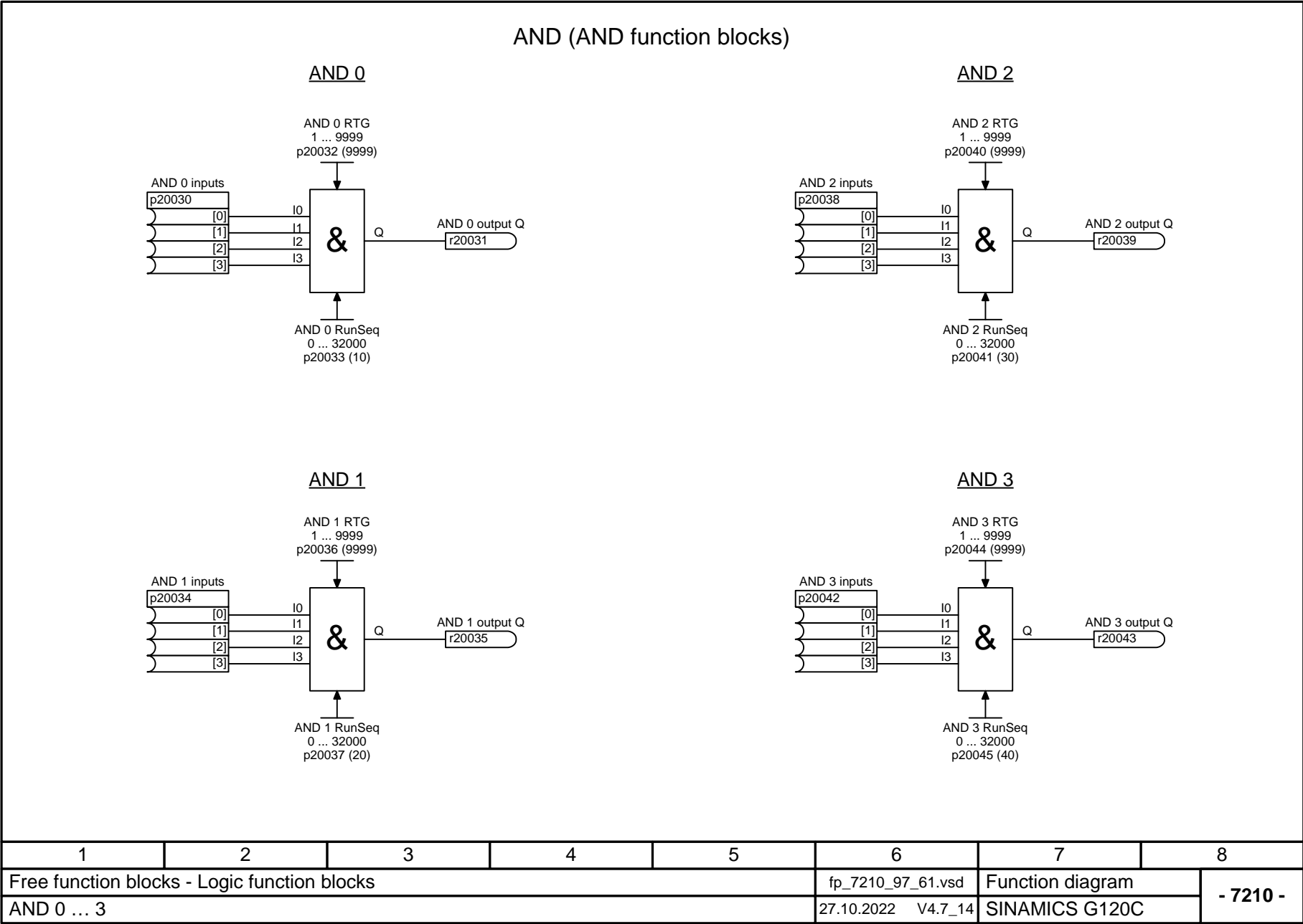
Fig. 3-127 7210 – AND 0 ... 3
