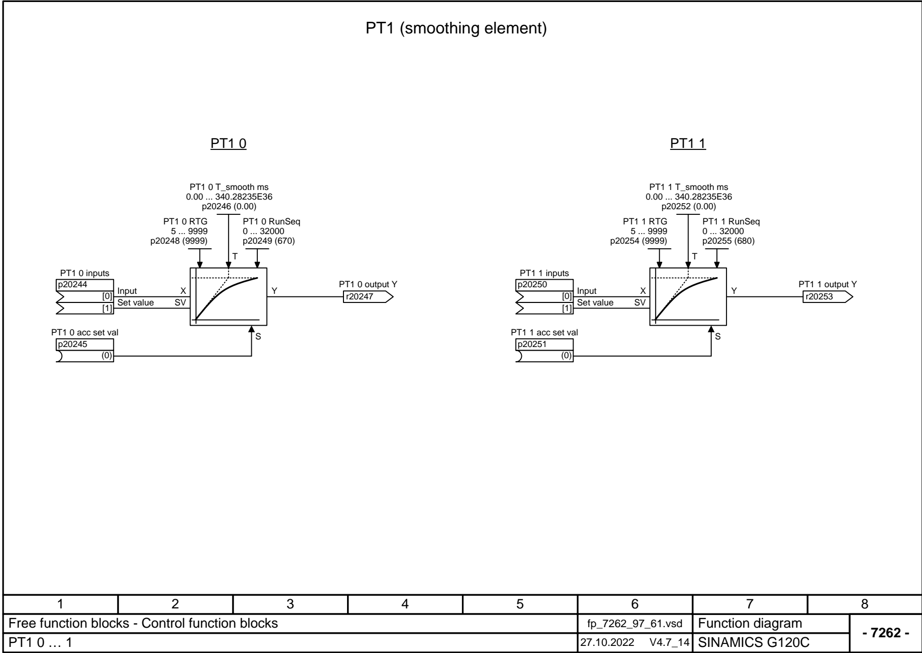
Fig. 3-143 7262 – PT1 0 ... 1
