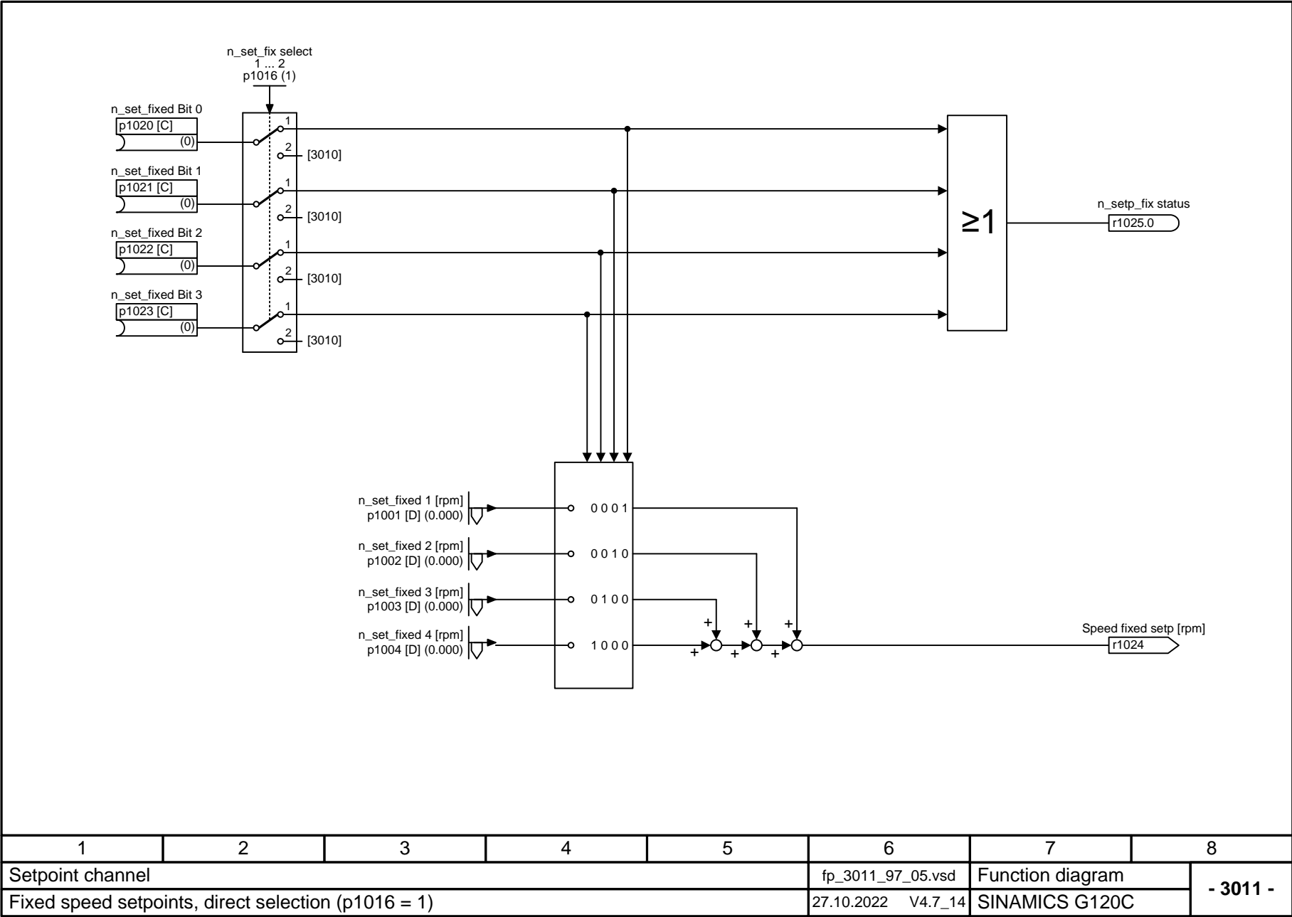
Fig. 3-66 3011 – Fixed speed setpoints, direct selection (p1016 = 1)
