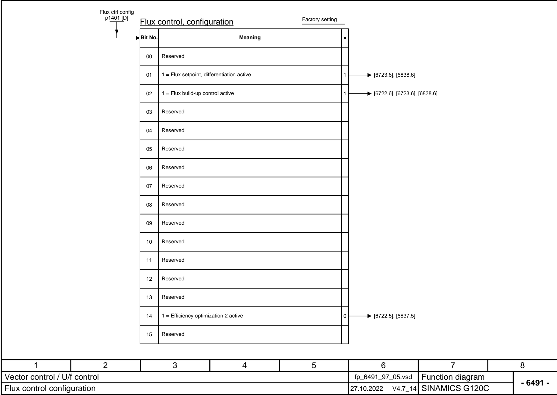
Fig. 3-84 6491 – Flux control configuration
