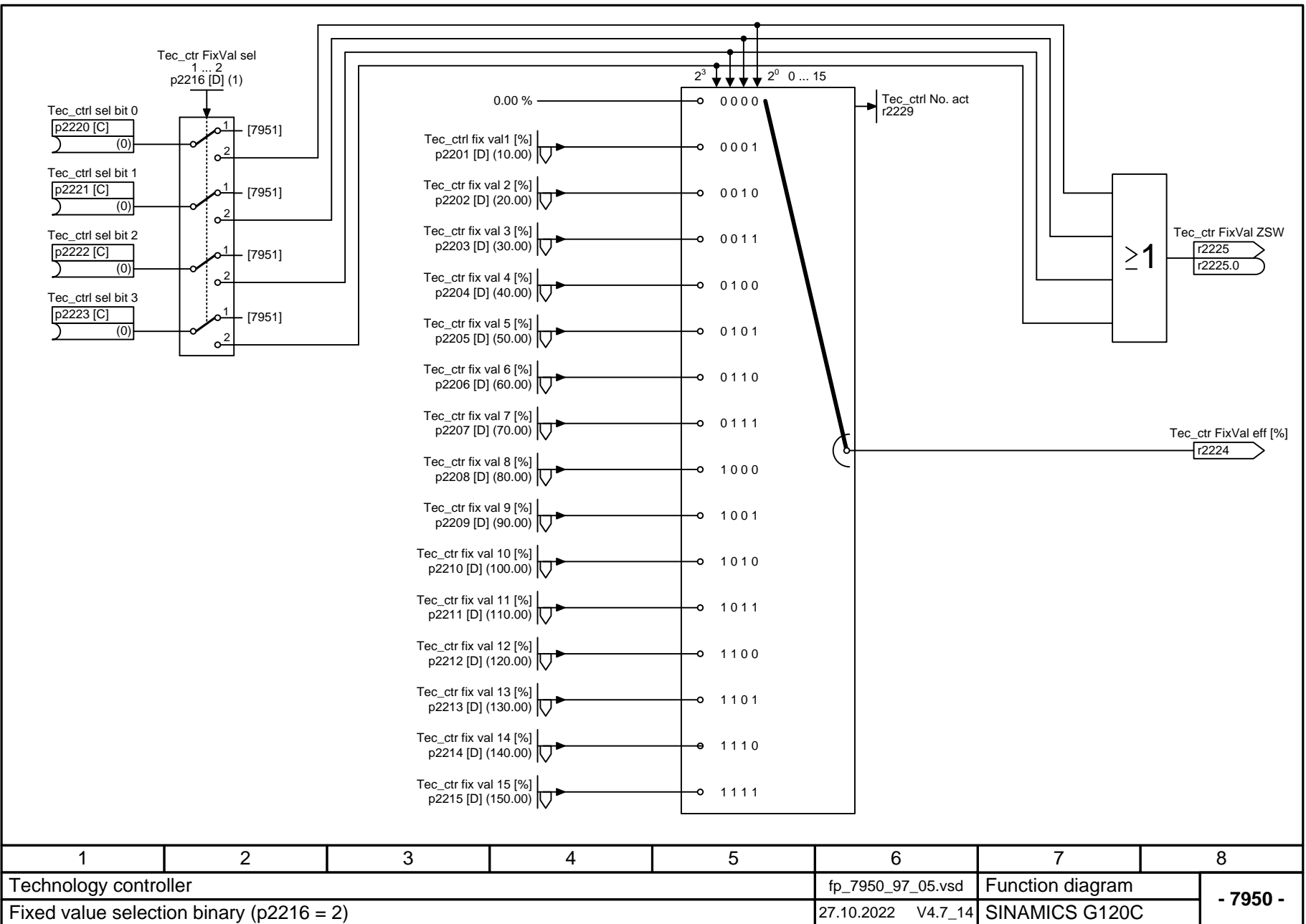
Fig. 3-146 7950 – Fixed values, binary selection (p2216 = 2)
