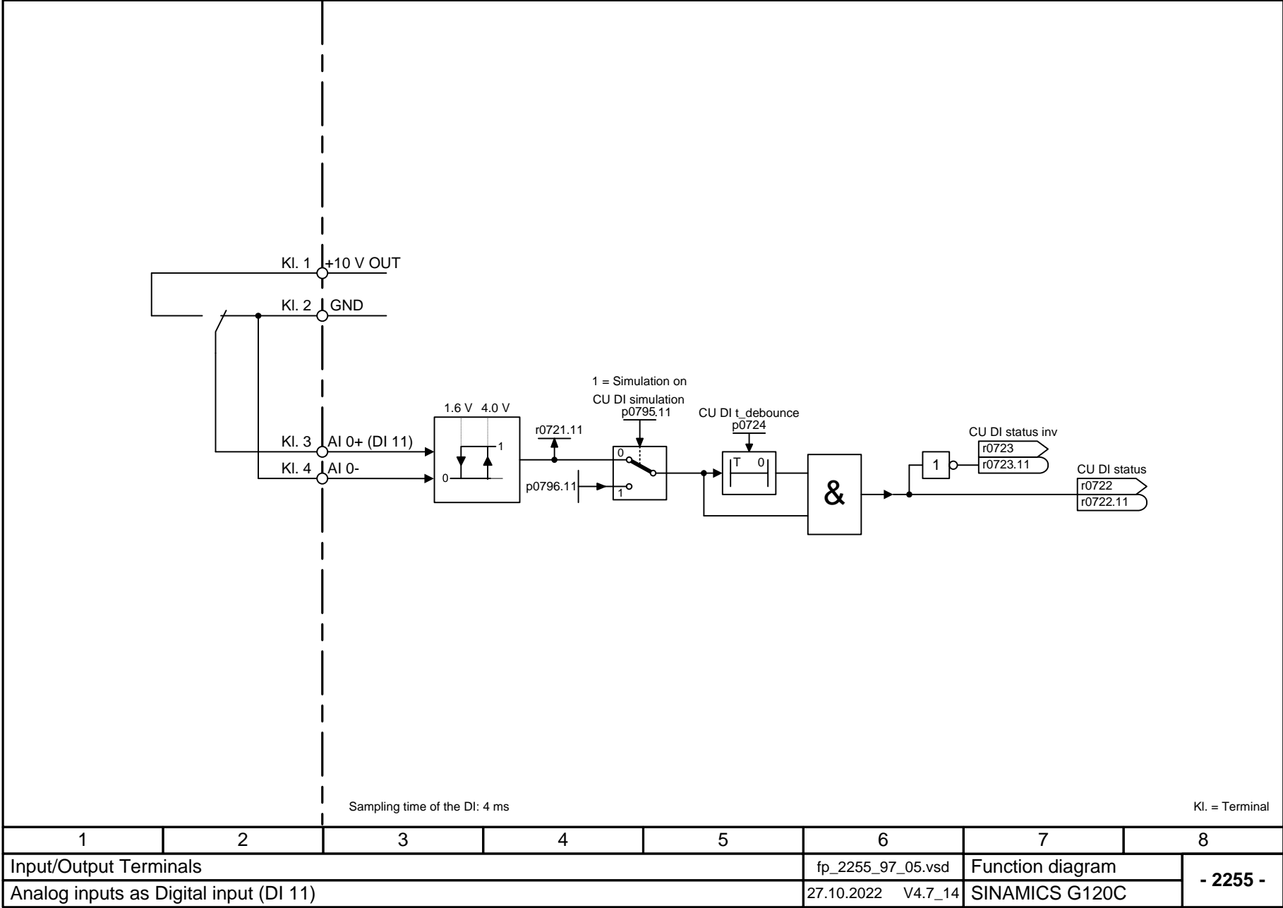
Fig. 3-9 2255 – Analog inputs as digital input (DI 11)
