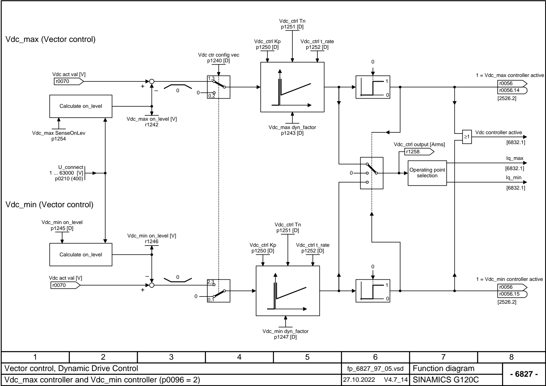
Fig. 3-111 6827 – Vdc_max controller and Vdc_min controller (p0096 = 2)
