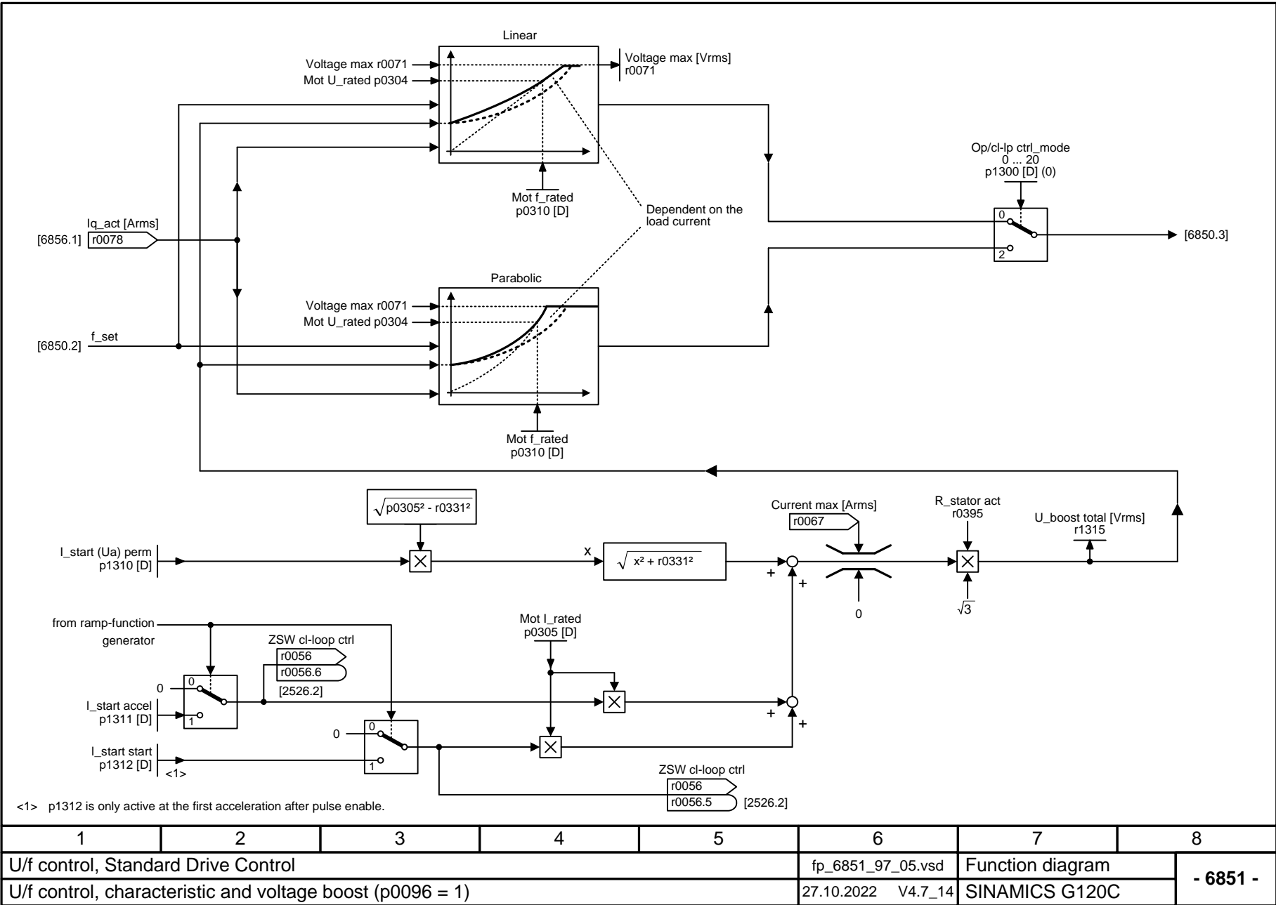
Fig. 3-101 6851 – U/f control, characteristic and voltage boost (p0096 = 1)
