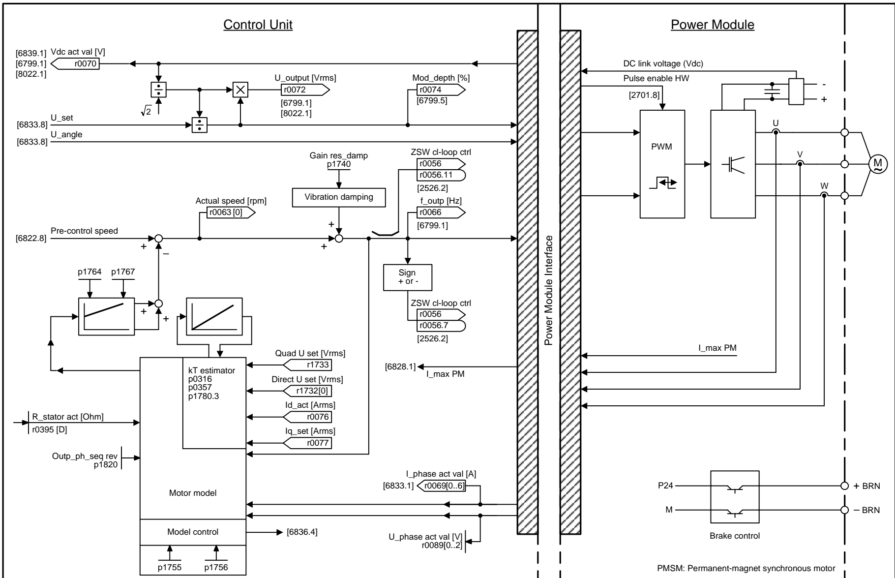
Fig. 3-122 6842 – Interface to the Power Module (PMSM, p0300 = 2xx, p0096 = 2)
