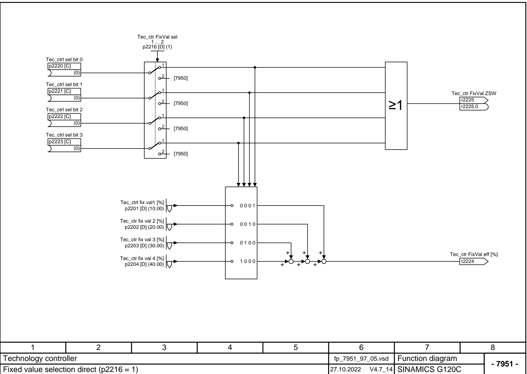
Fig. 3-147 7951 – Fixed values, direct selection (p2216 = 1)
