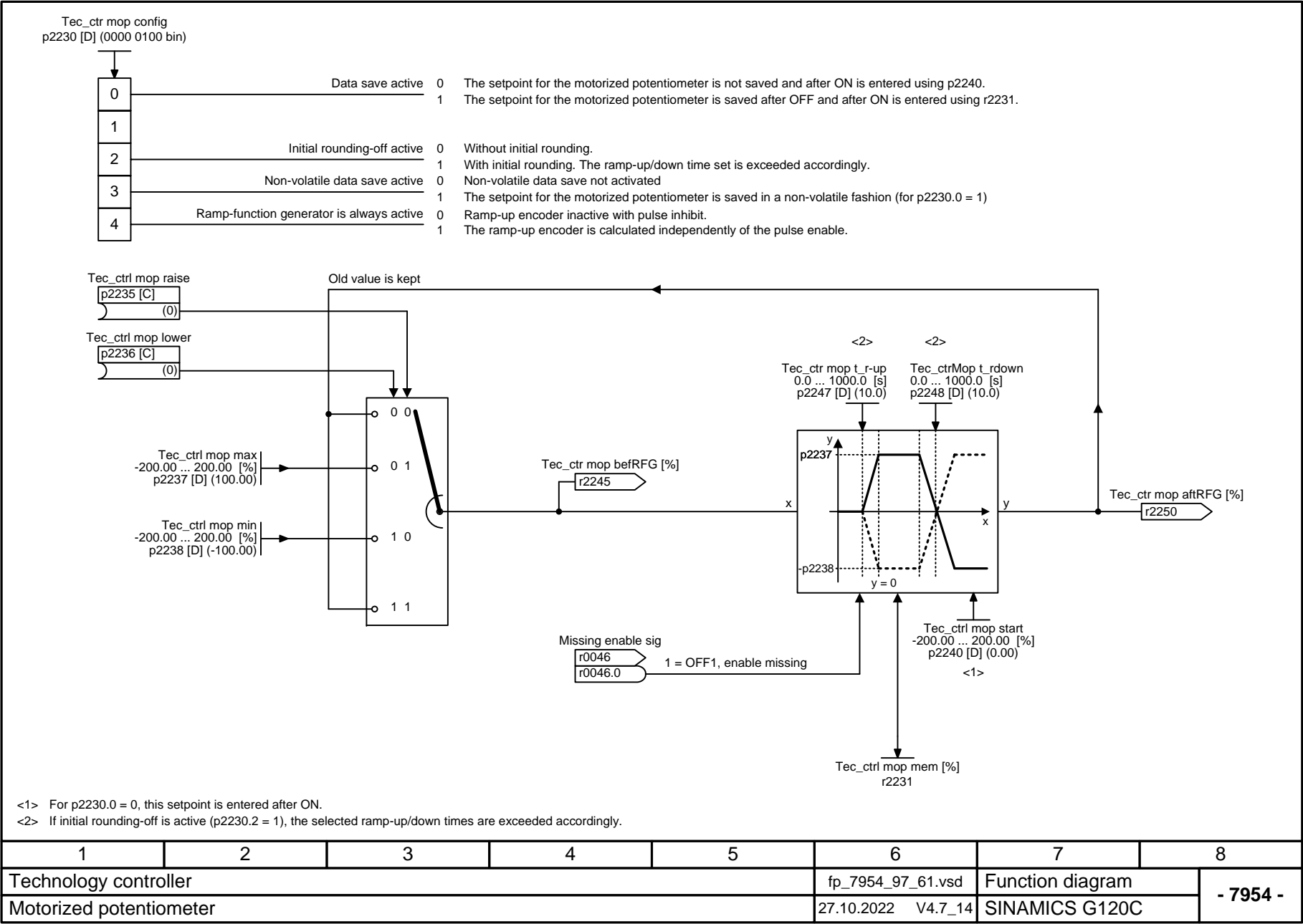
Fig. 3-148 7954 – Motorized potentiometer
