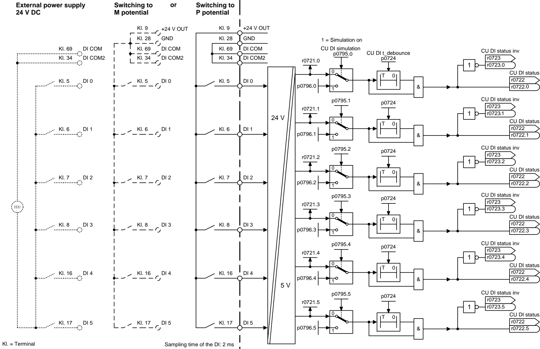
2221 – Digital inputs, electrically isolated (DI 0 ... DI 5)
