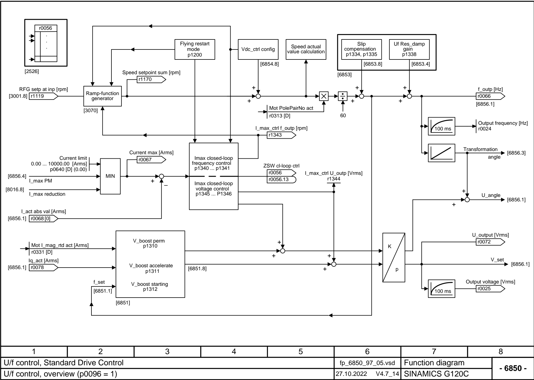
Fig. 3-100 6850 – U/f control, overview (p0096 = 1)
