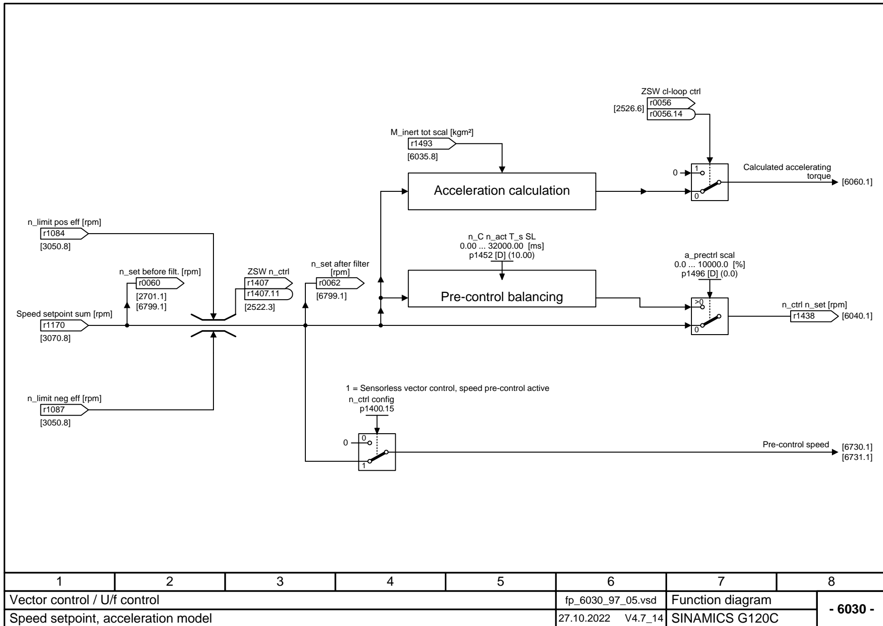
Fig. 3-74 6030 – Speed setpoint, acceleration model
