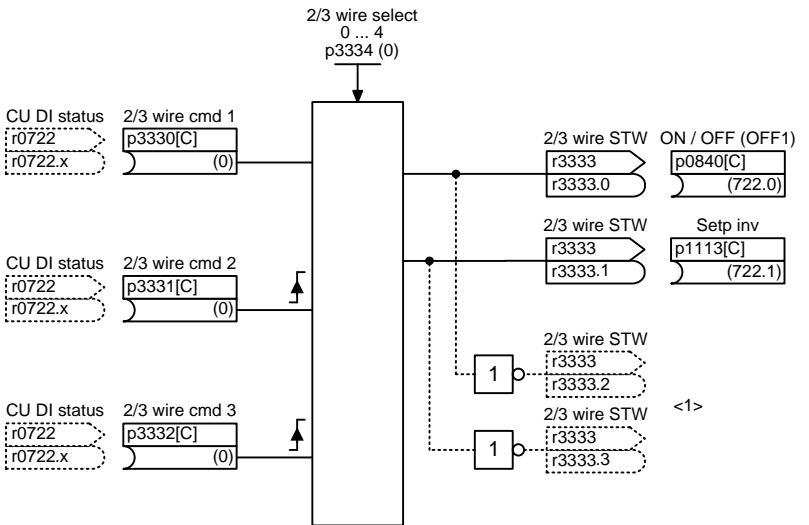
Fig. 3-12 2273 – Three-wire control
