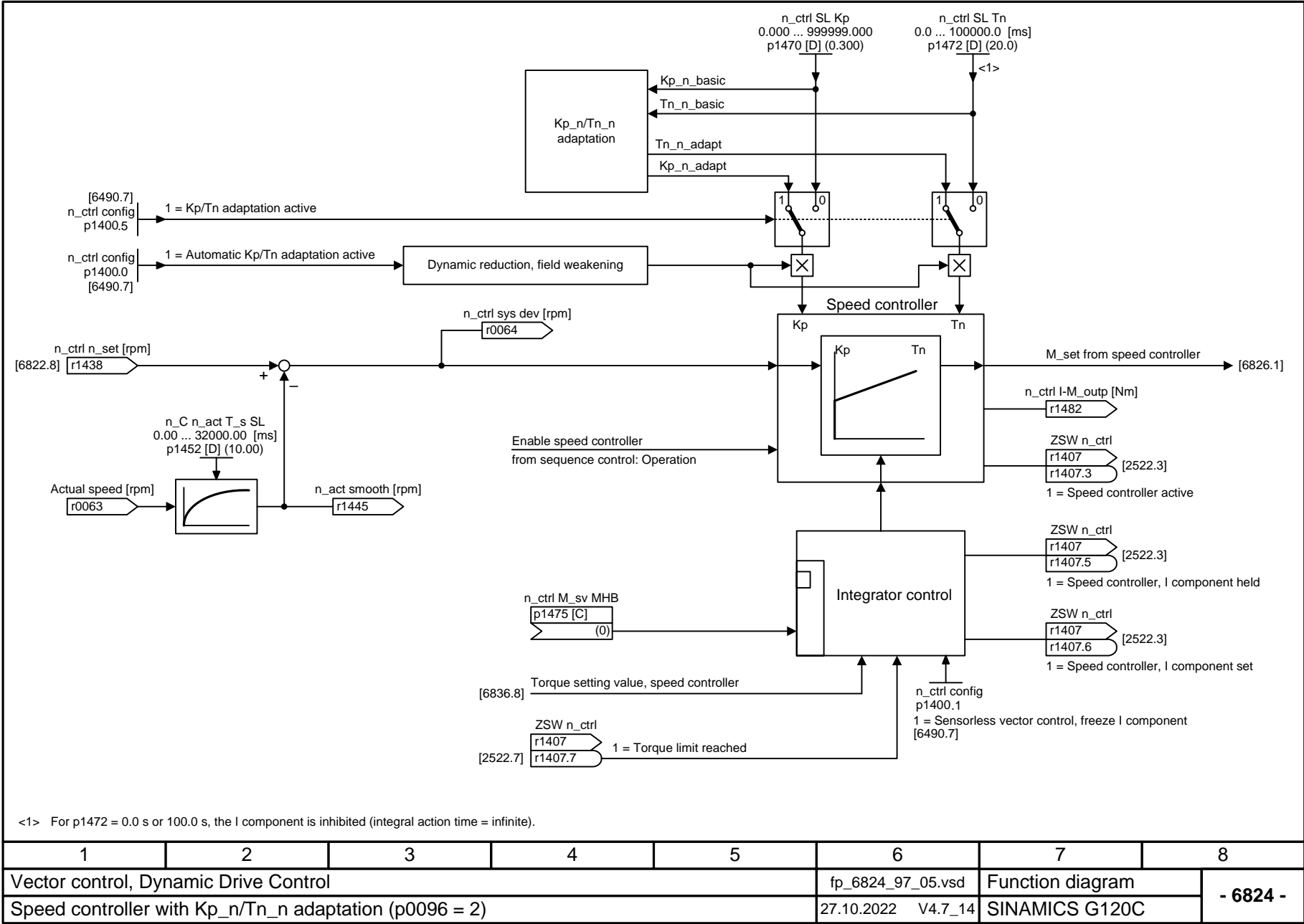
Fig. 3-109 6824 – Speed controller with Kp_n/Tn_n adaptation (p0096 = 2)
