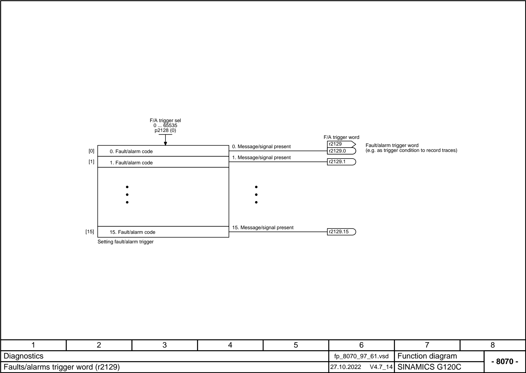
Fig. 3-164 8070 – Faults/alarms trigger word (r2129)
