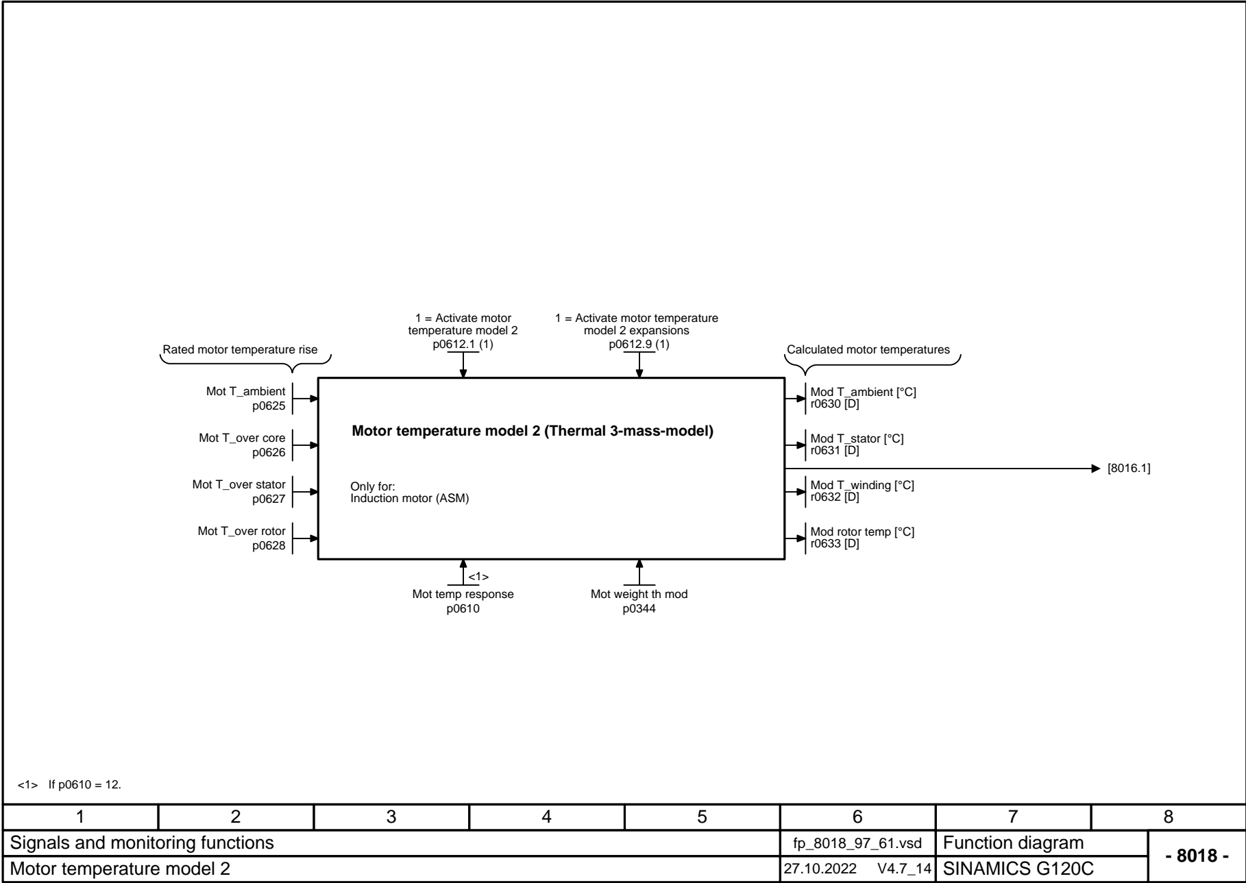
Fig. 3-156 8018 – Motor temperature model 2
