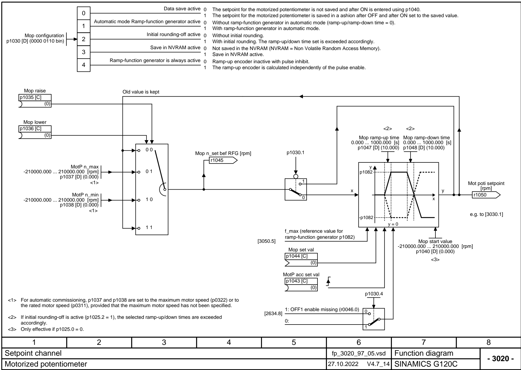
Fig. 3-67 3020 – Motorized potentiometer
