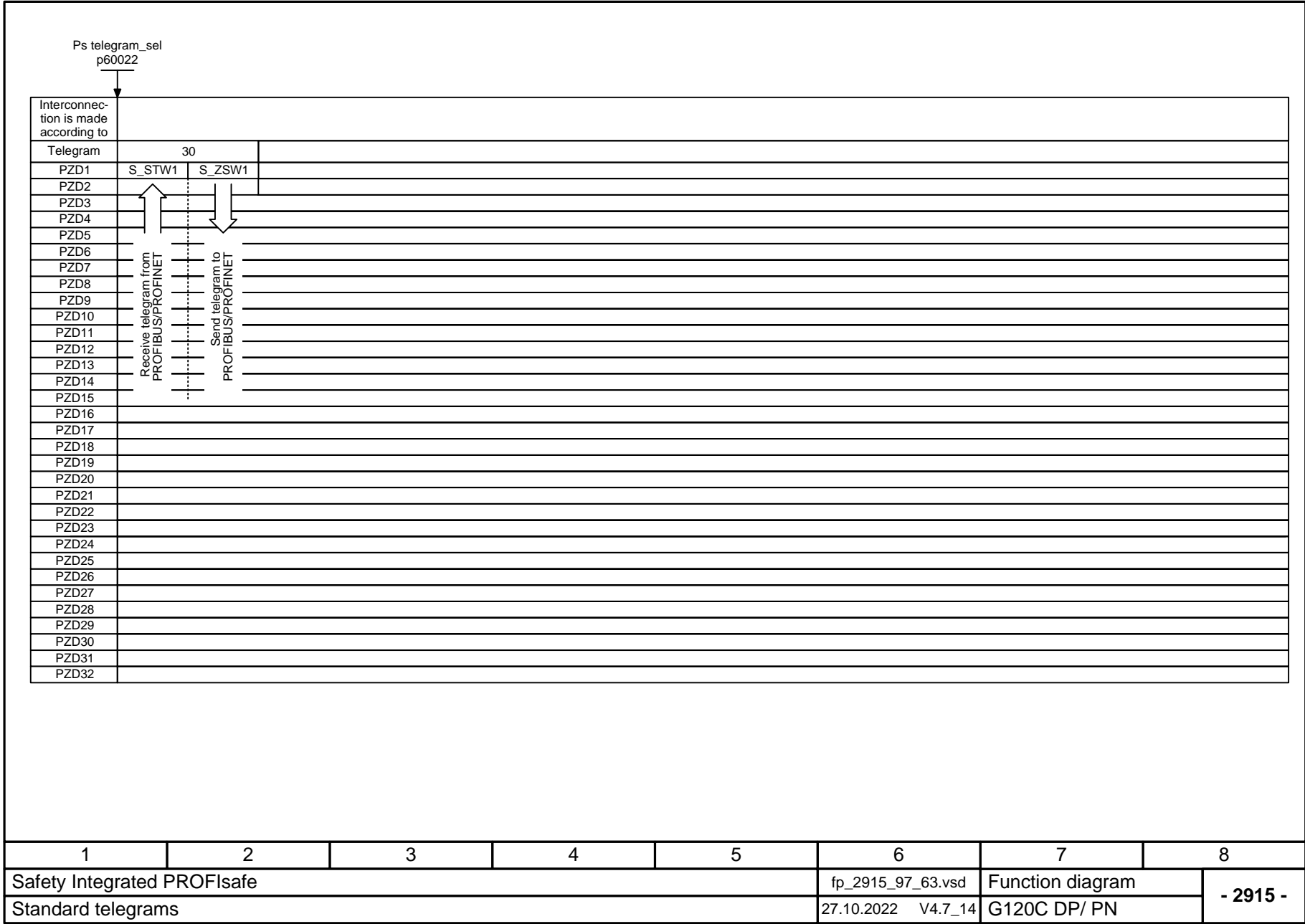
Fig. 3-63 2915 – Standard telegrams
