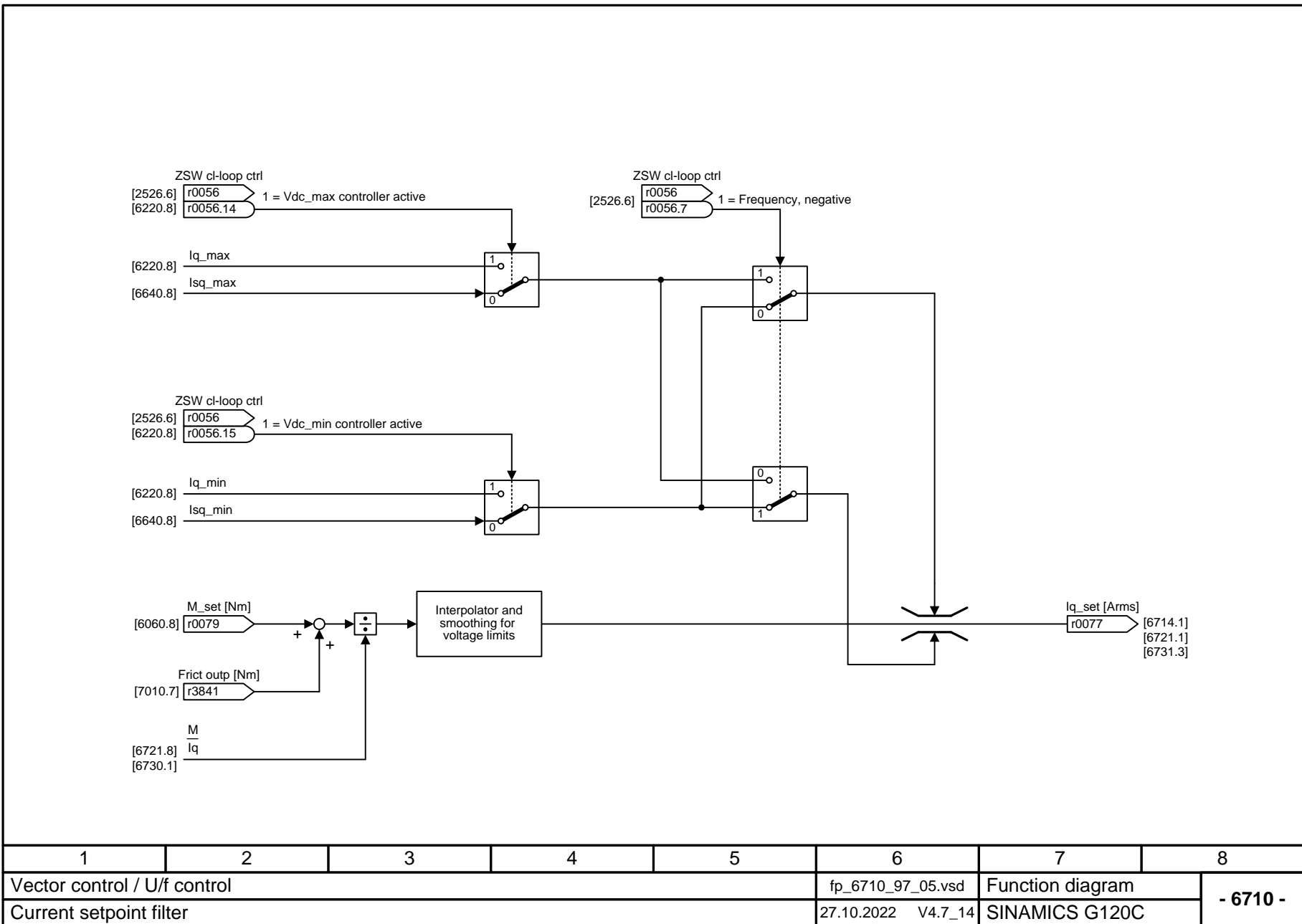
Fig. 3-88 6710 – Current setpoint filter
