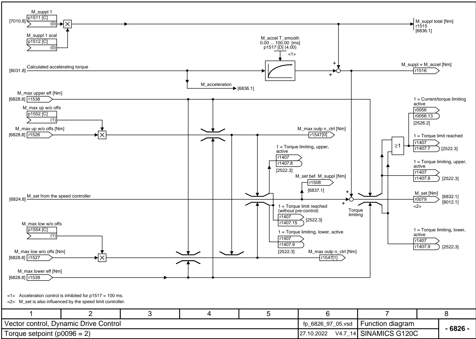
Fig. 3-110 6826 – Torque setpoint (p0096 = 2)
