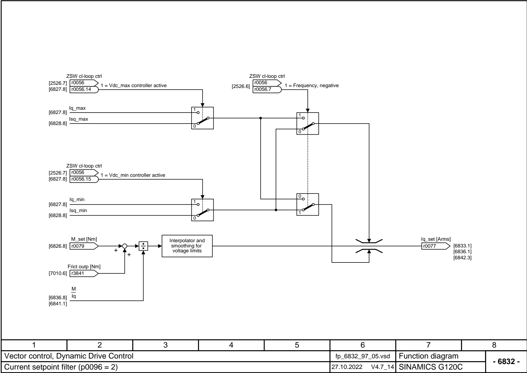
Fig. 3-113 6832 – Current setpoint filter (p0096 = 2)
