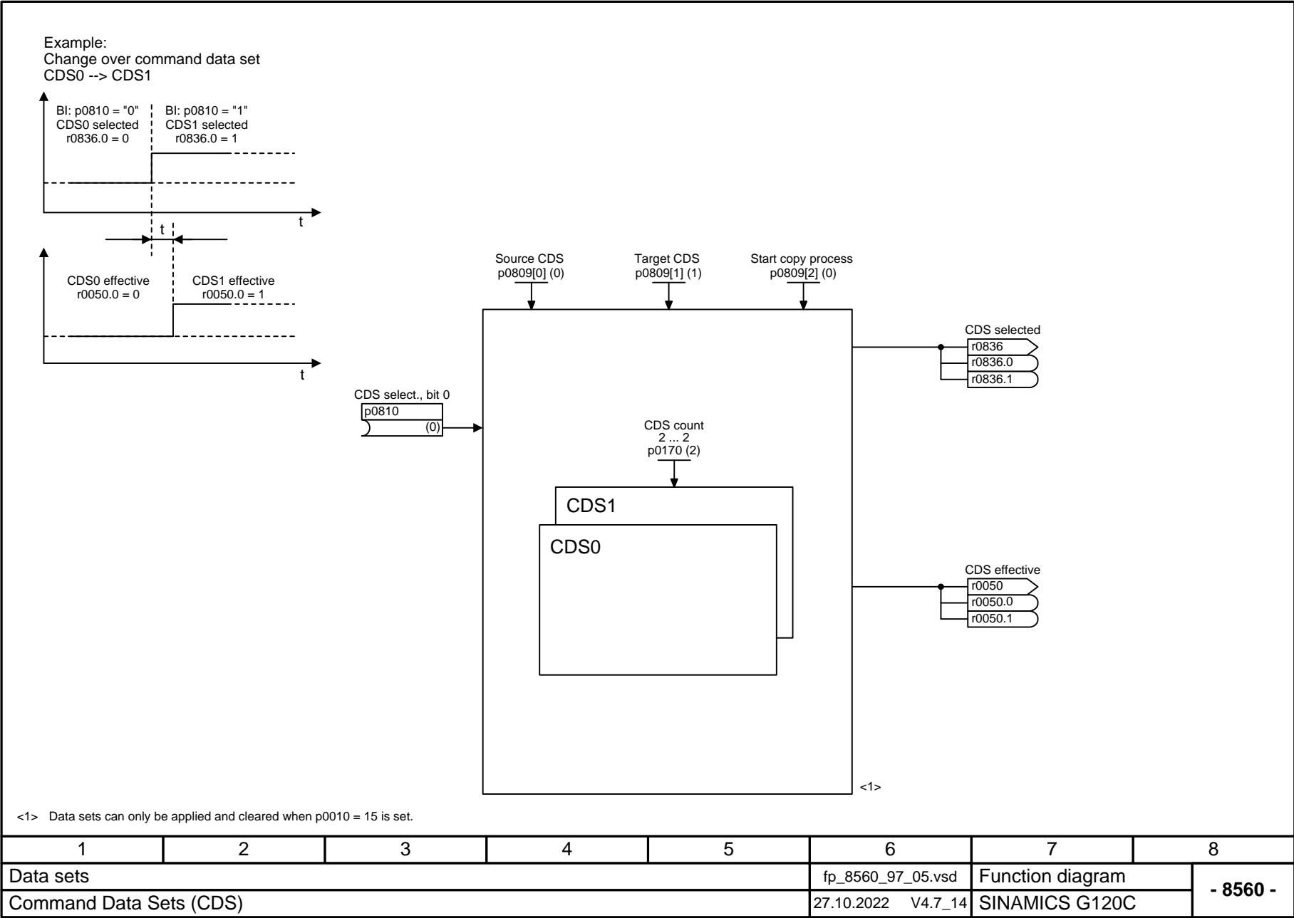
Fig. 3-166 8560 – Command Data Sets (CDS)
