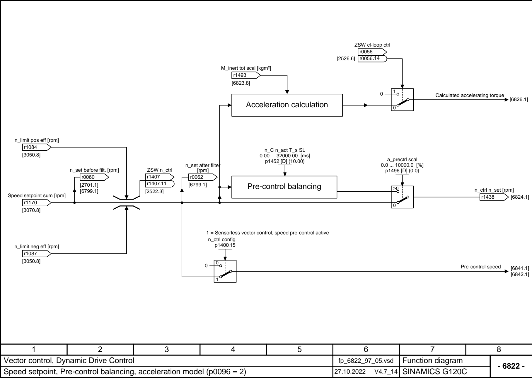
Fig. 3-107 6822 – Speed setpoint, precontrol symmetrization, acceleration model (p0096 = 2)
