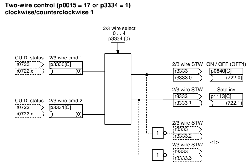
Fig. 3-11 2272 – Two-wire control
