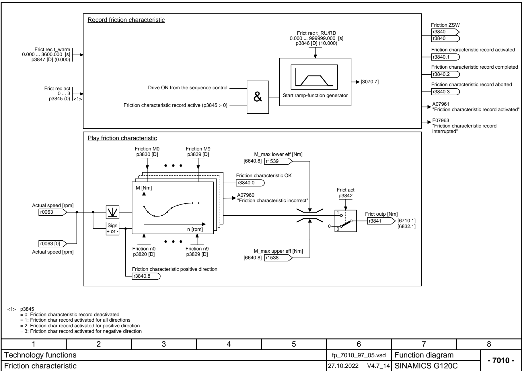
Fig. 3-124 7010 – Friction characteristic
