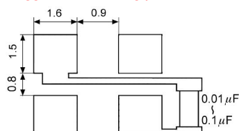
Suggested soldering pad:
