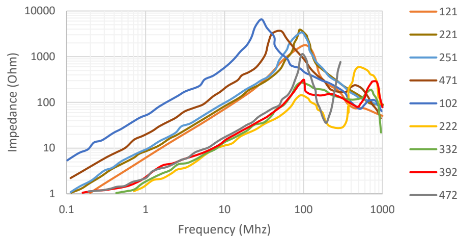
ACMS-1065 Differential Mode Impedance
