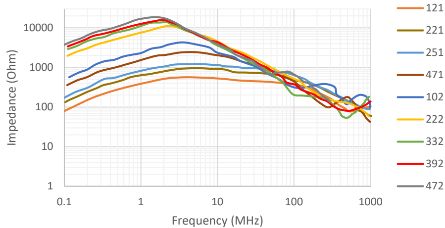
ACMS-1065 Common Mode Impedance
