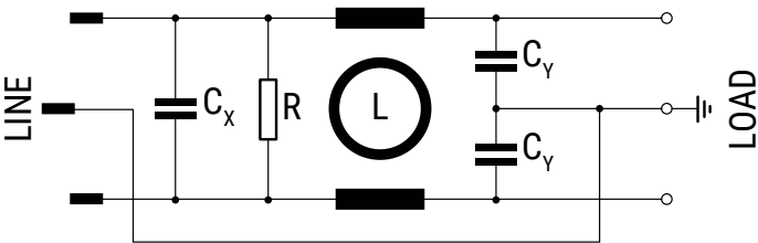
Circuit Diagram
