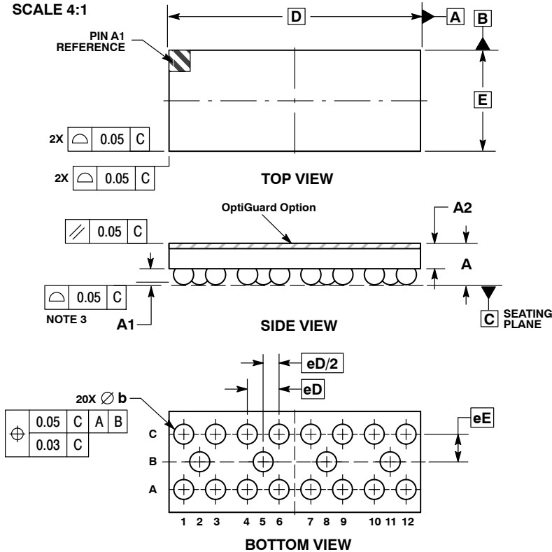
WLCSP20, 3.96x1.59 CASE 567BY ISSUE O
