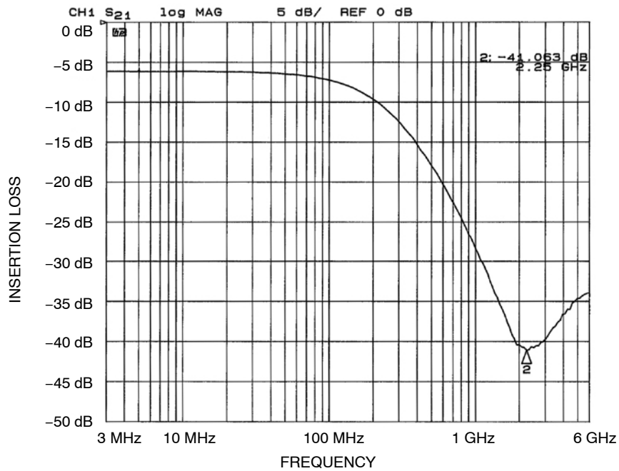
Figure 8. Insertion Loss vs. Frequency (FILTER4 Input to GND, CM1630-06DE)
