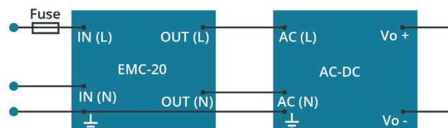
Figure 2 Application Circuit
