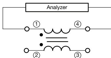
DC Resistance
