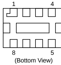
Figure 3. Pin Diagram
