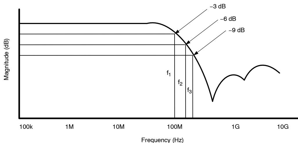
Figure 8. Filter Bandwidth
